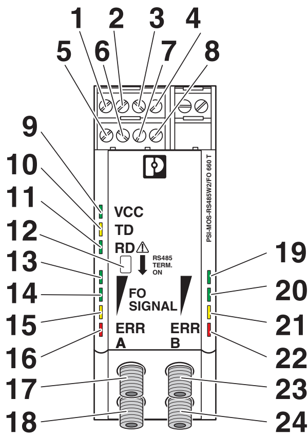
Schematic diagram
