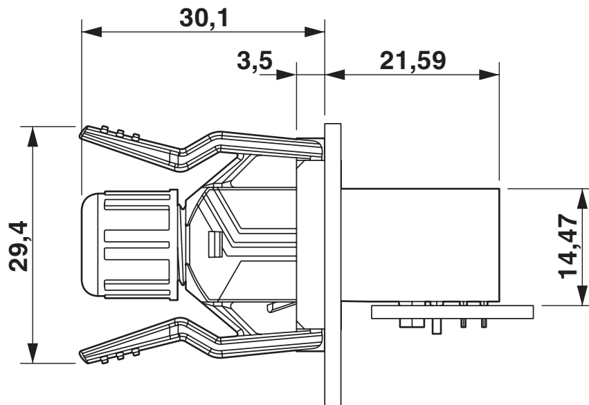
Dimensional drawing
