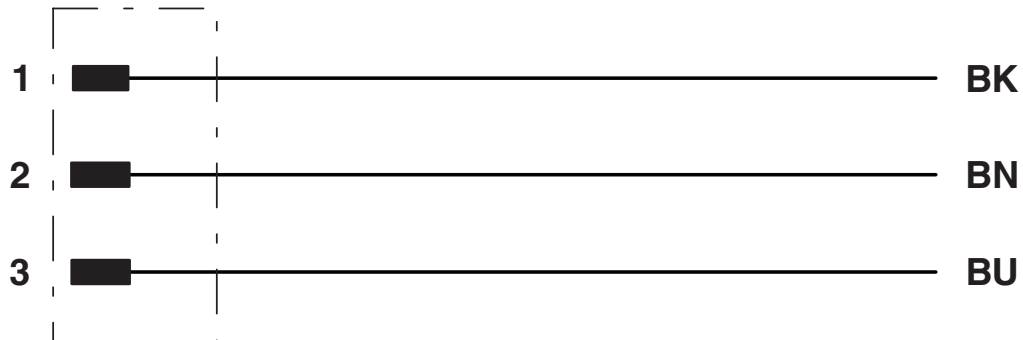
Circuit diagram
