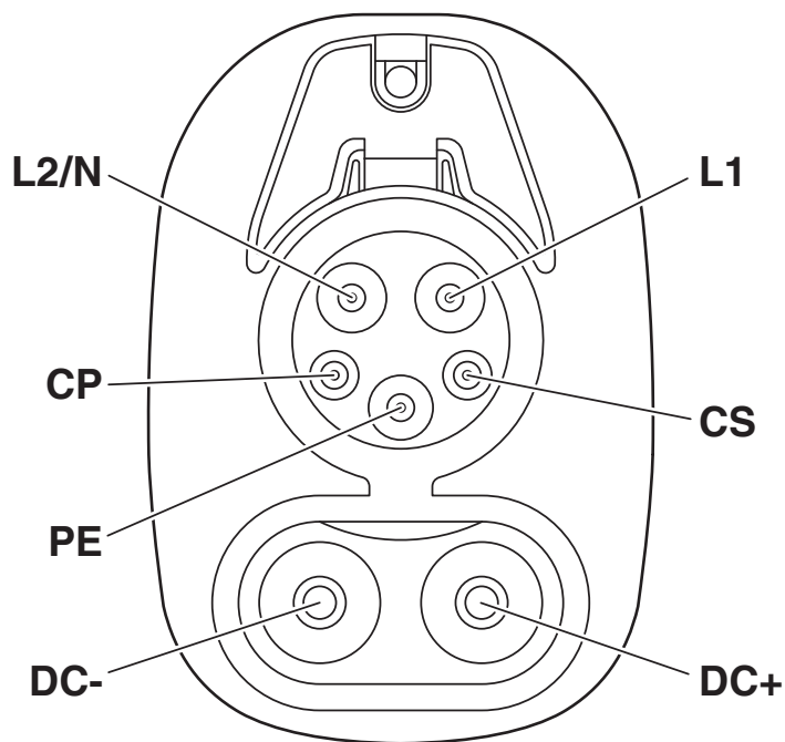
Connection diagram
