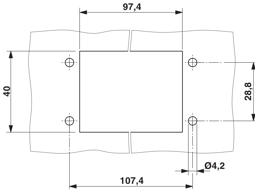
Dimensional drawing
