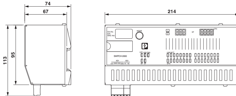
Dimensional drawing
