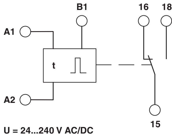
Block diagram
