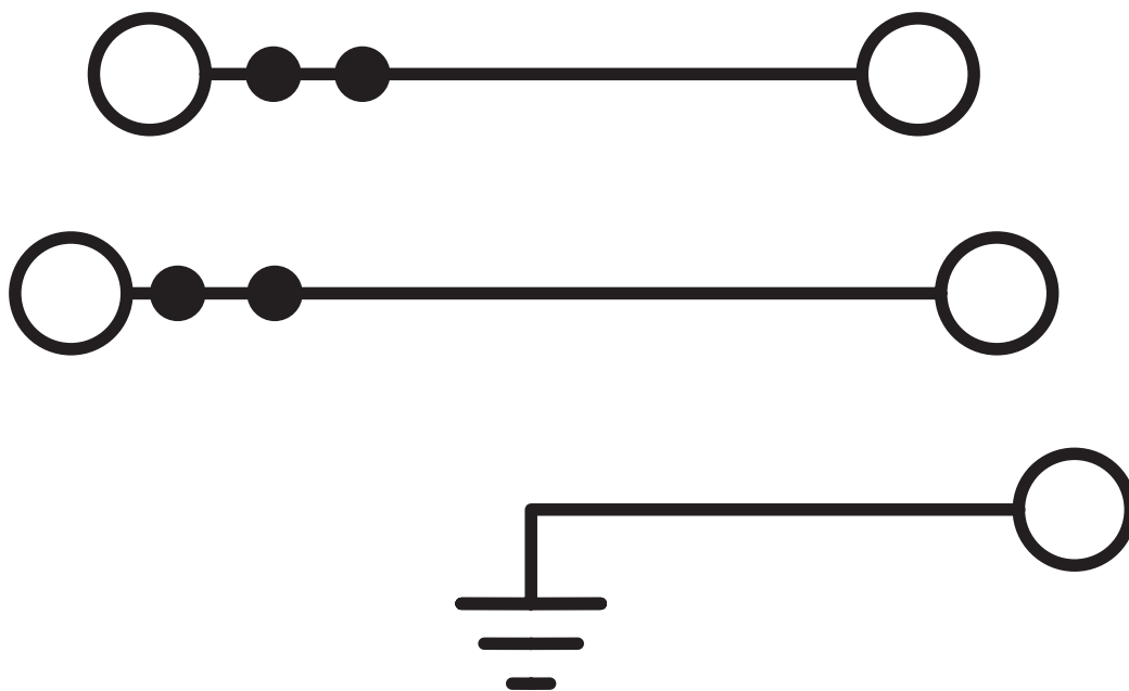
Circuit diagram
