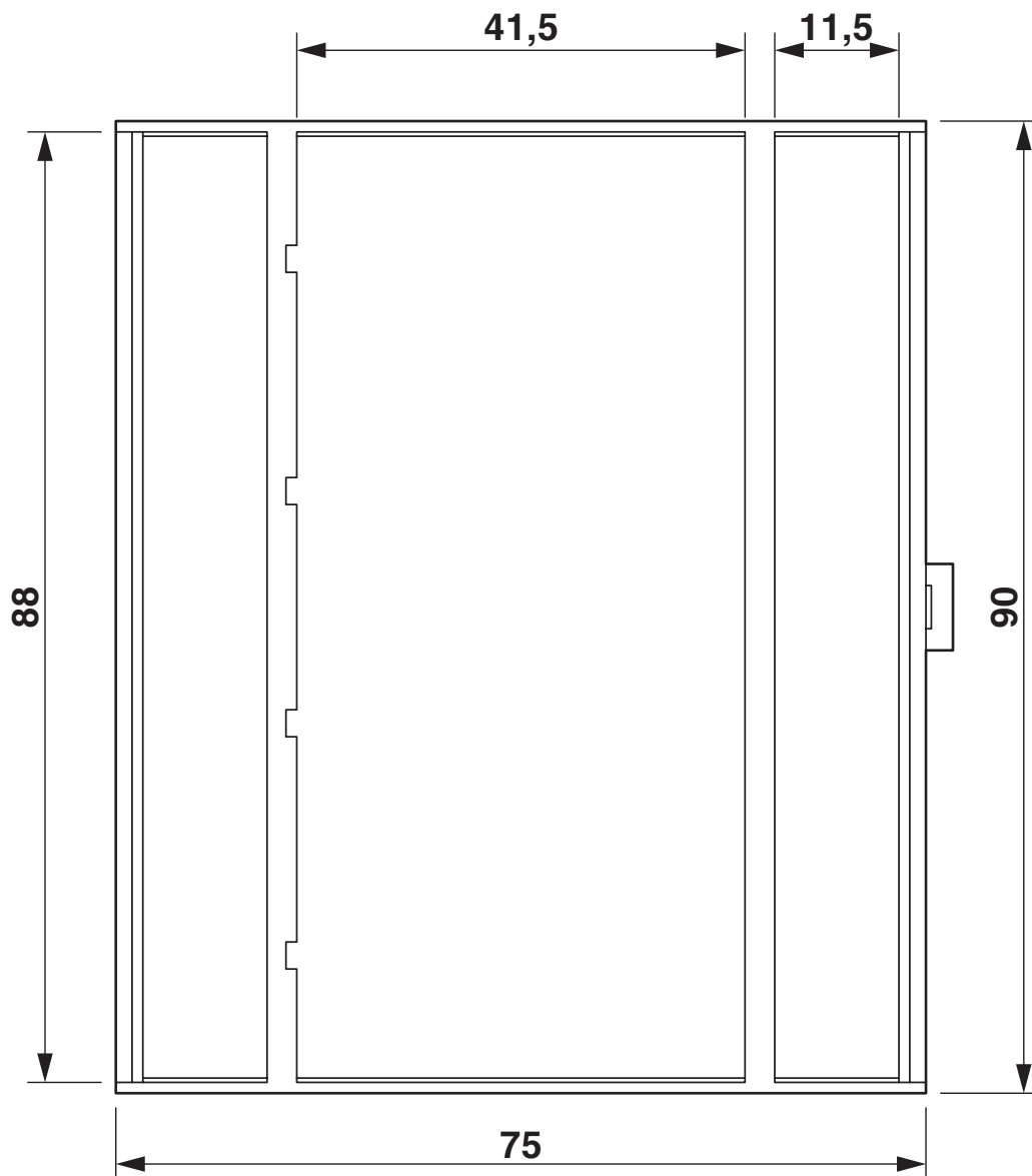
Dimensional drawing
