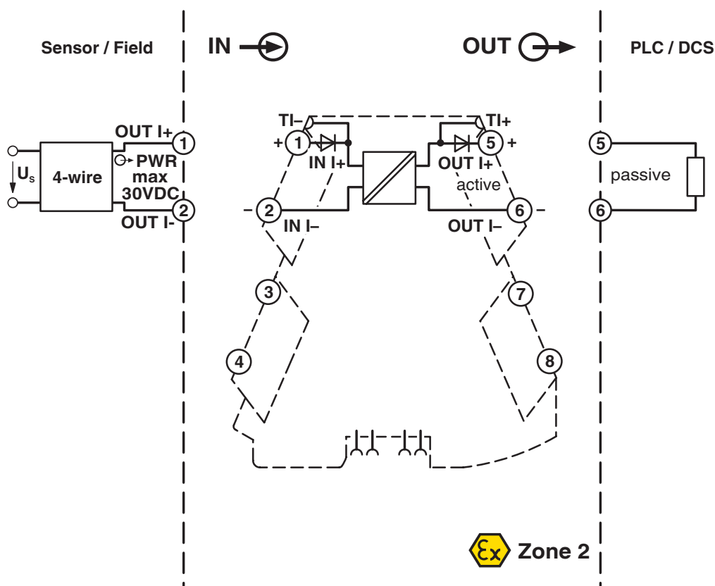
Block diagram
