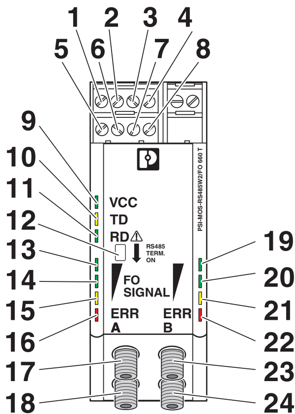
Schematic diagram
