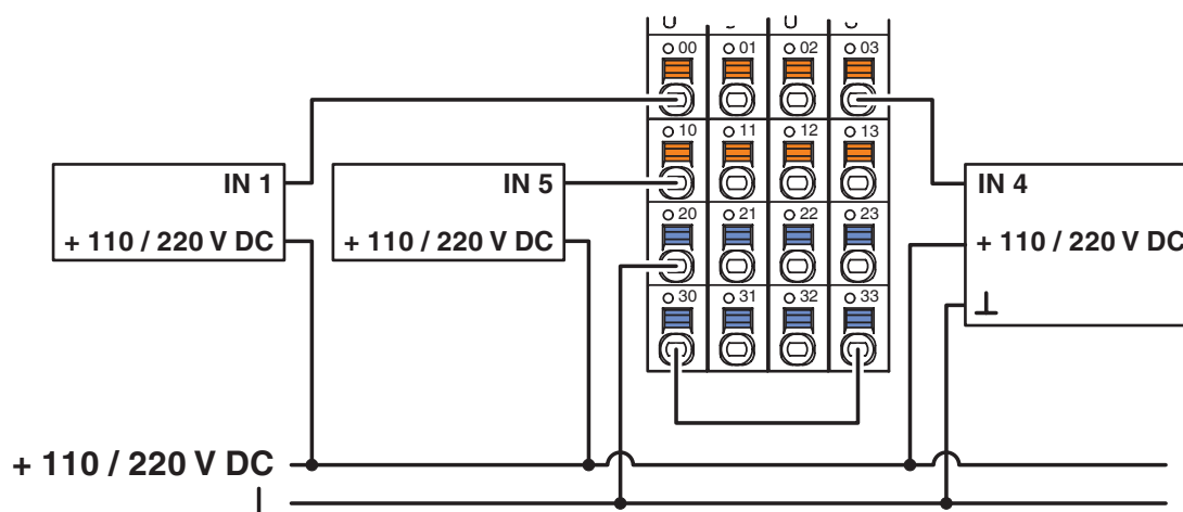
Connection diagram
