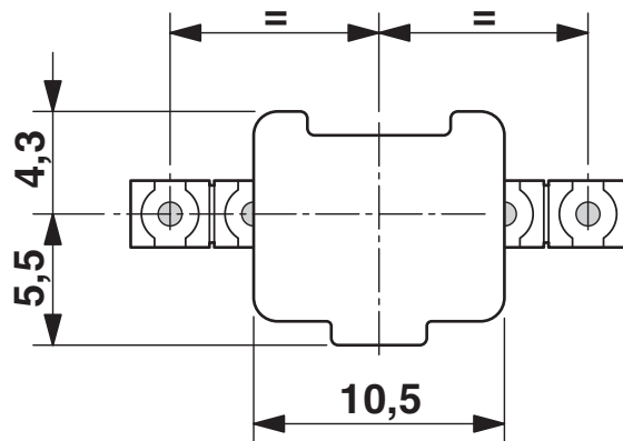
Dimensional drawing
