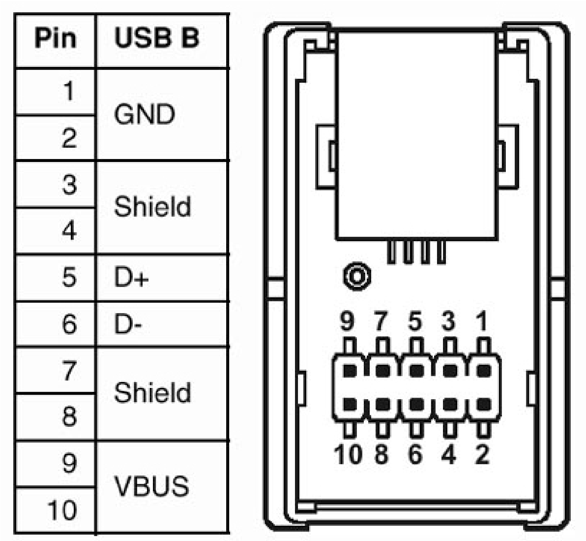
Contact assignment
