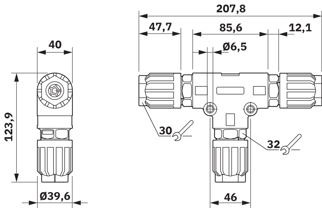
Dimensional drawing
