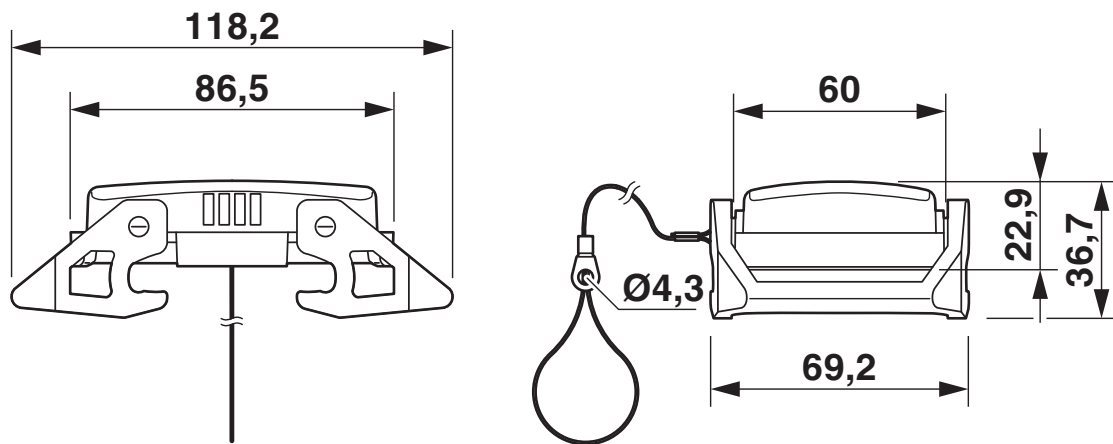
Dimensional drawing
