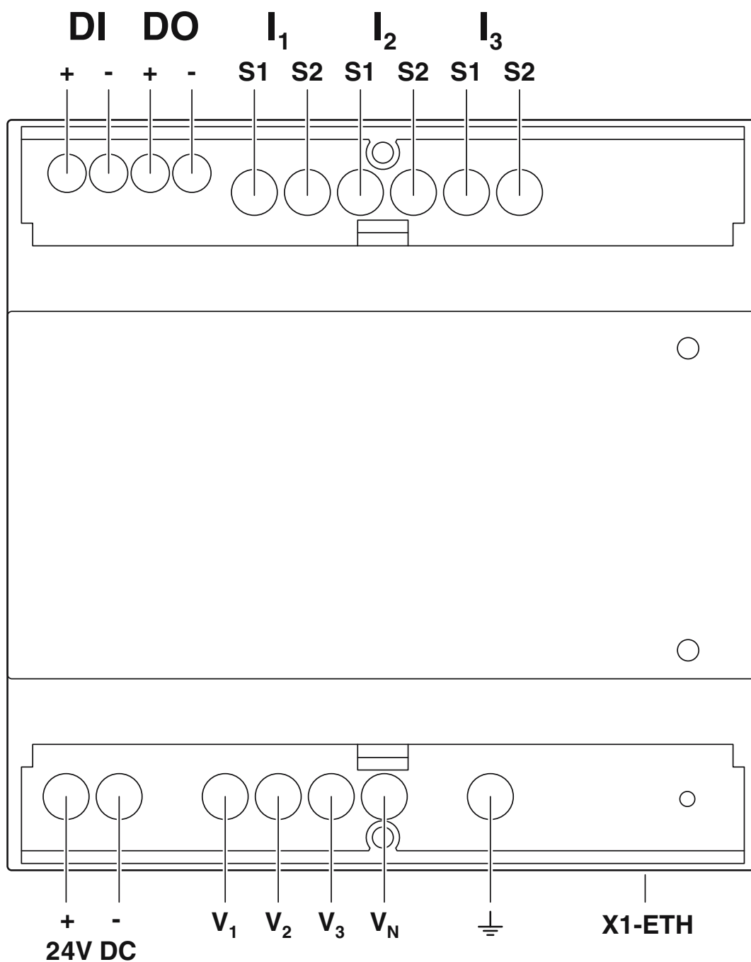
Connection diagram
