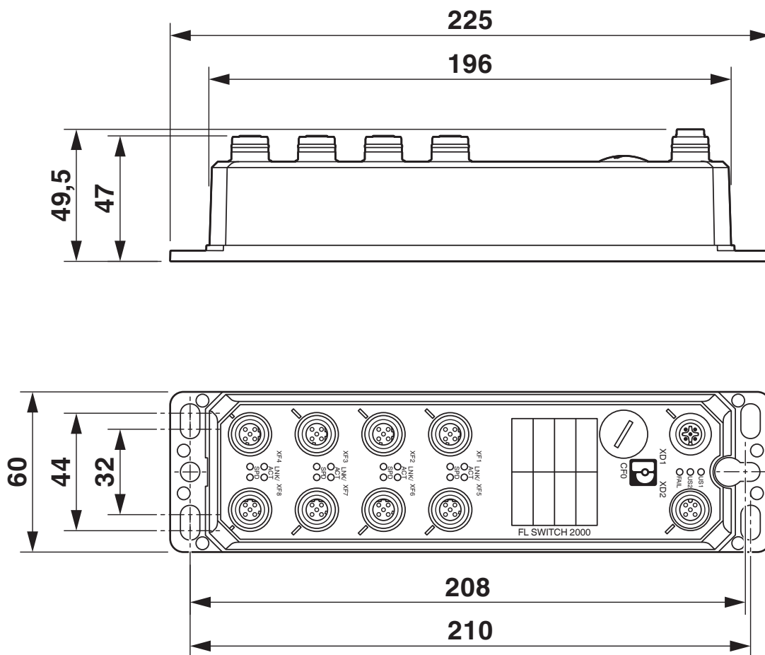
Dimensional drawing
