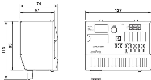
Dimensional drawing
