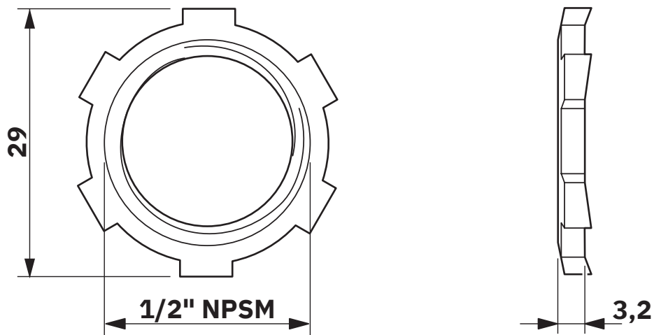
Dimensional drawing
