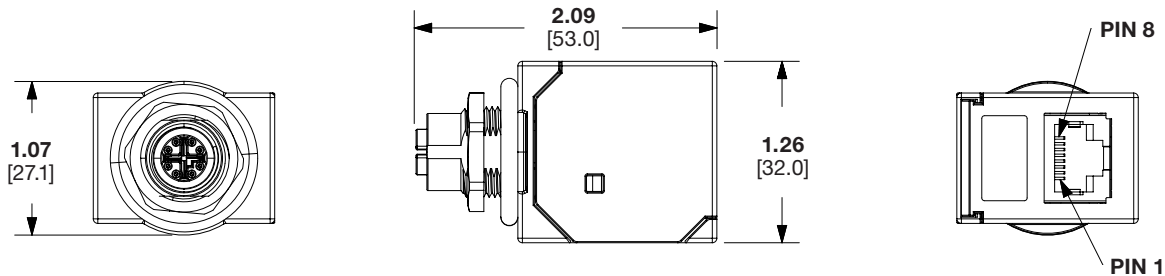
ICAM12X90RJS - Industrial M12 X-Code, 8 pin Female to RJ45 Cat 6A Jack 90-Degree
