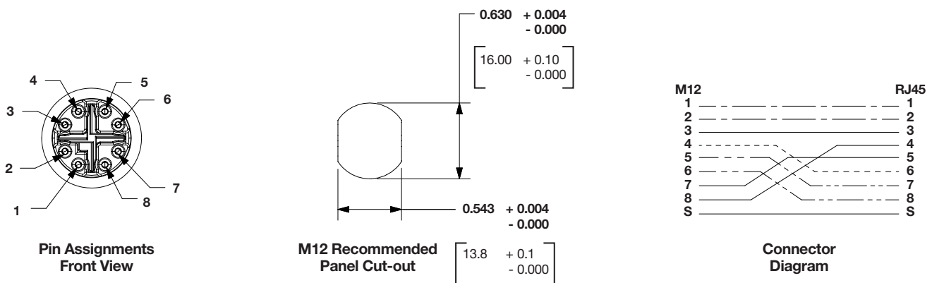
Pin Assignments and Recommended M12 Panel Cut-Out
