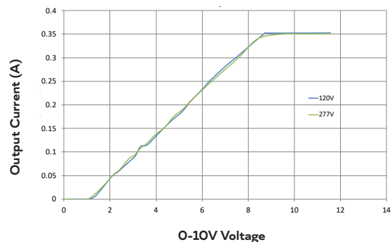
Dimming Curve
