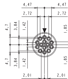
12-14 14 contacts 14xØ1.0 (#20)
