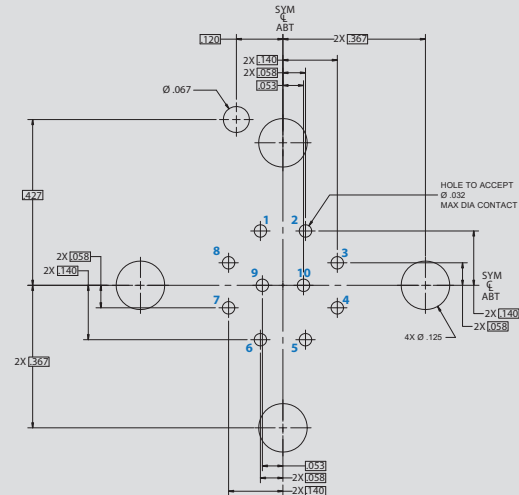
Arrangement No. 11-10 10x #20HD Contacts
