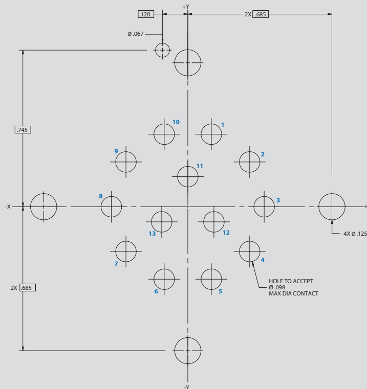
Arrangement No. 22-13 13x #12 Contacts
