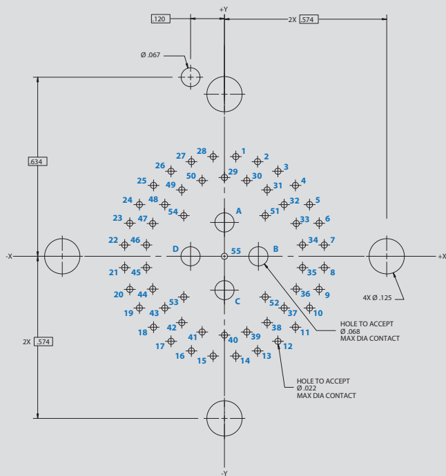
Arrangement No. 18-59 4x #16 and 55x #22HD Contacts
