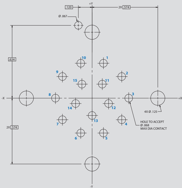
Arrangement No. 18-15 15x #16 Contacts
