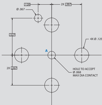
Arrangement No. 8-1 1x #16 Contacts
