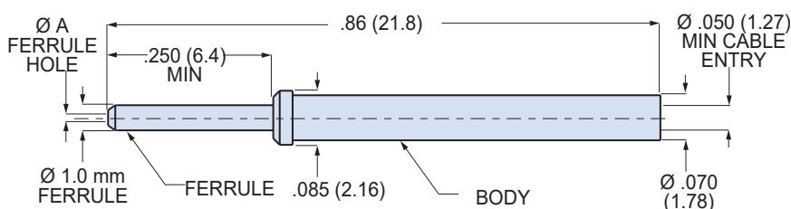
#20HD Pin Terminus 181-134
