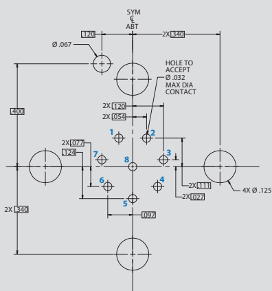
Arrangement No. 10-8 8x #20HD Contacts
