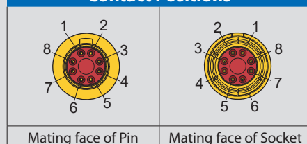
El Ochito® Red for SATA 3.0 100 Ohm Datalinks, pin contact mating face
