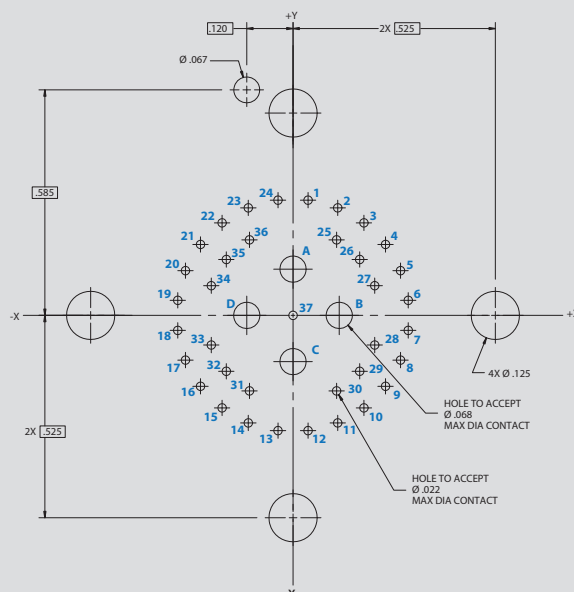
4x #16 and 37x #22HD Contacts
