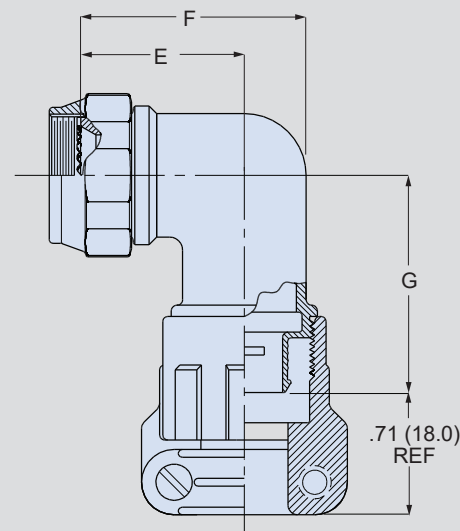
4470VW1061 90°
