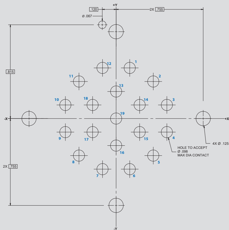
Arrangement No. 24-19 19x #12 Contacts
