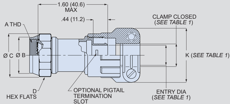
4470VS1061 STRAIGHT
