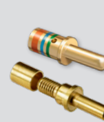
Size 12 Power, and RF Contacts
