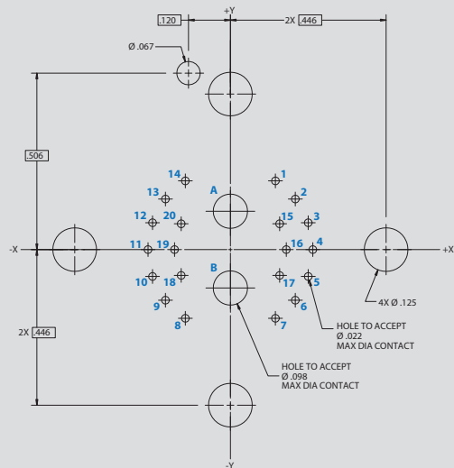
Arrangement No. 14-22 2x #12 and 20x #22HD Contacts
