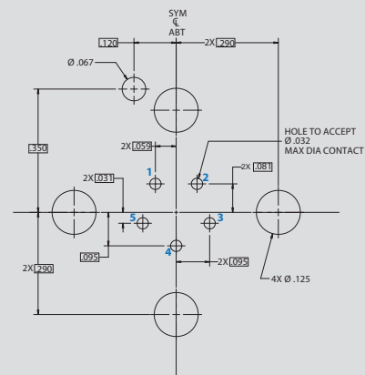
Arrangement No. 9-5 5x #20HD Contacts
