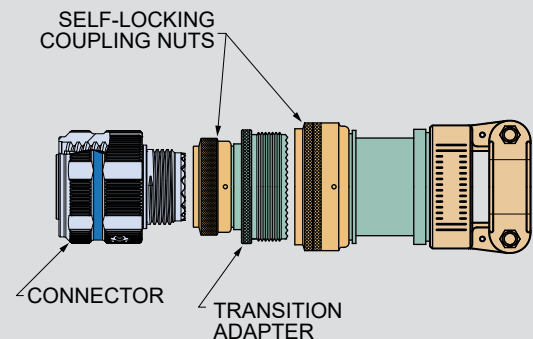
Style 2 Backshell
