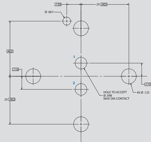
Arrangement No. 12-2 2x #12 Contacts
