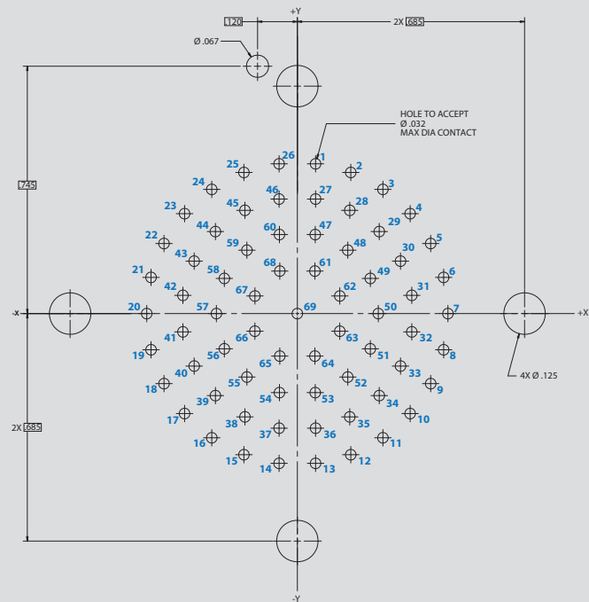
Arrangement No. 22-69 69x #20HD Contacts
