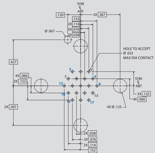
Arrangement No. 11-19 19x #22HD Contacts
