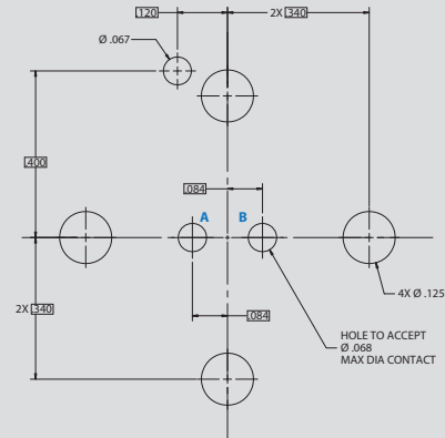
Arrangement No. 10-2 2x #16 Contacts
