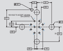
Printed Circuit Board Layouts Page 159
