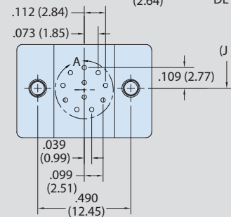
ARRANGEMENT NO. 9-11 11 X #22HD CONTACTS PIN FACE SHOWN (SOCKET FACE OPPOSITE)
