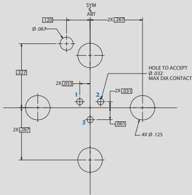
Arrangement No. 8-3 3x #20HD Contacts
