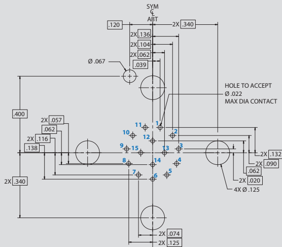
Arrangement No. 10-15 15x #22HD Contacts
