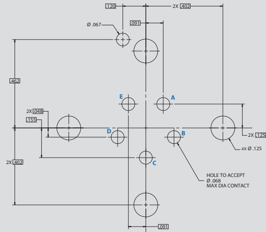
Arrangement No. 12-5 5x #16 Contacts
