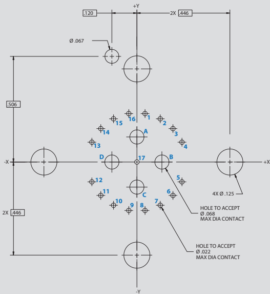
Arrangement No. 14-21 4x #16 and 17x #22HD Contacts
