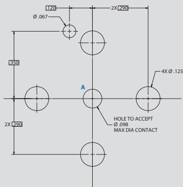
Arrangement No. 9-1 1x #12 Contact
