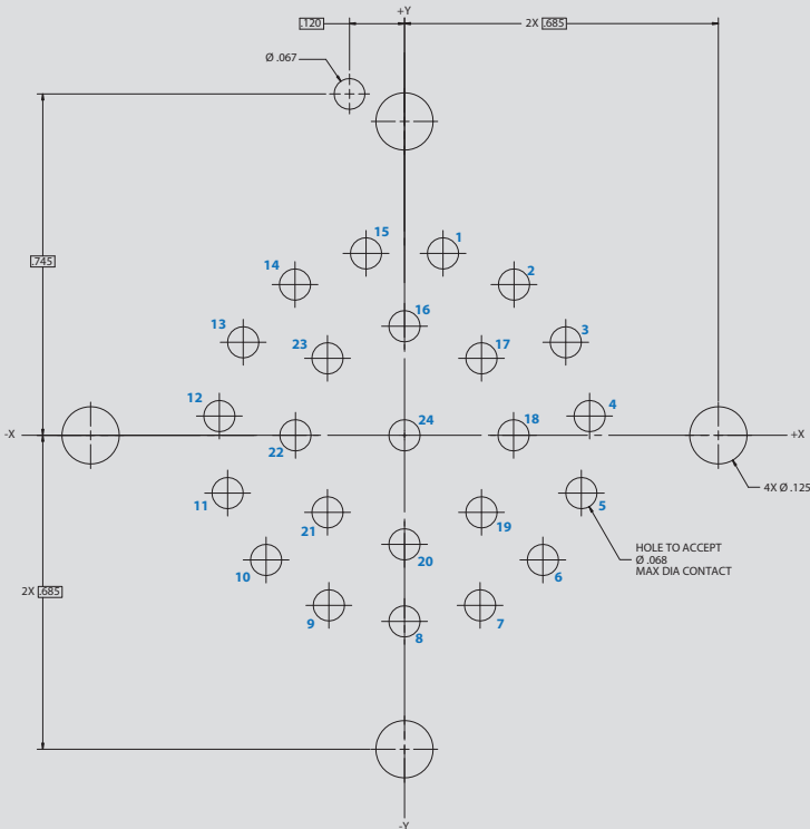
Arrangement No. 22-24 24x #16 Contacts
