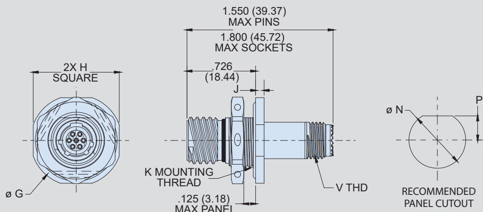
806-087-07 Jam-Nut Mount Receptacle Dimensions
