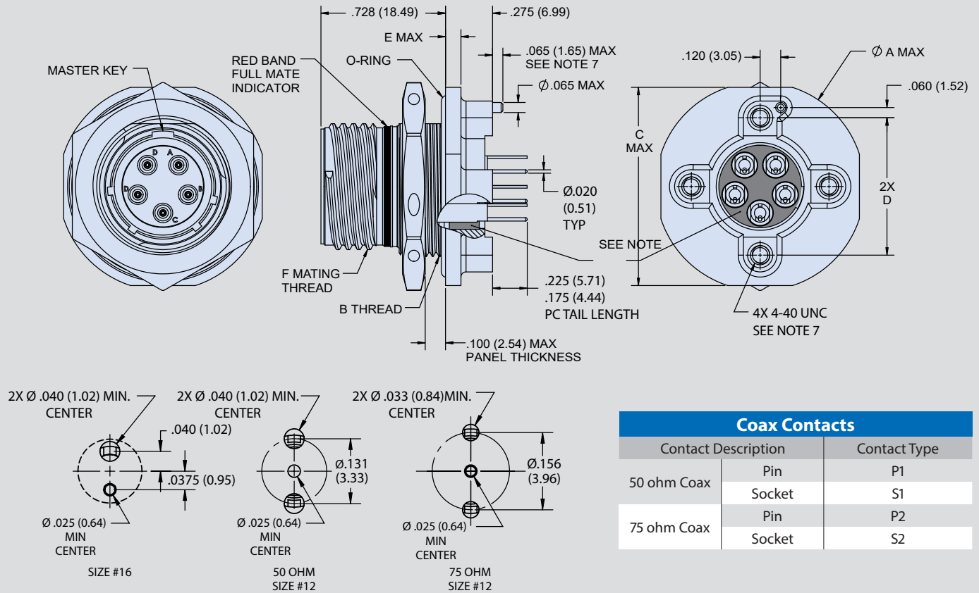
COAX PCB FOOTPRINT
