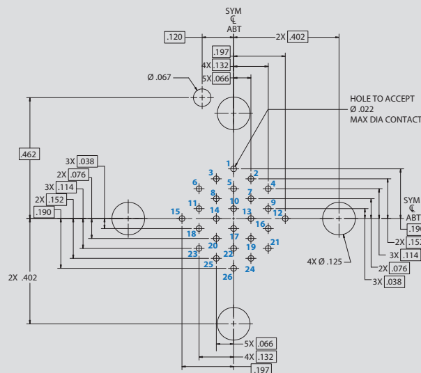
Arrangement No. 12-26 26x #22HD Contacts
