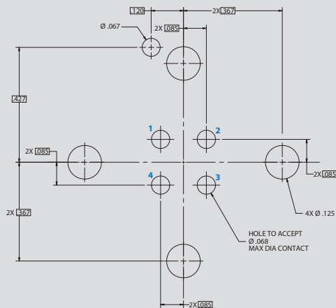
Arrangement No. 11-4 4x #16 Contacts
