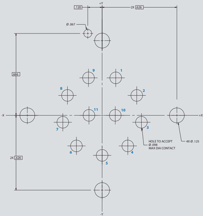
Arrangement No. 20-11 11x #12 Contacts
