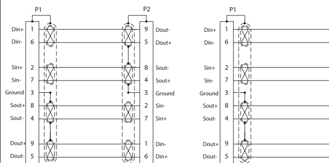
BACK TO BACK WIRING CABLE ASSY TYPE -AL ECSS-E-ST-50-12C REV 1, FIGURE 5-5
