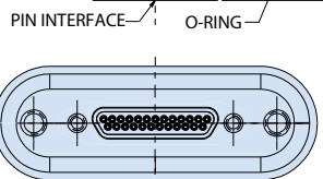
PIN-PIN (PP)
