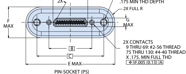
PIN-SOCKET (PS)
