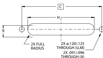
PIN-SOCKET (PS)
