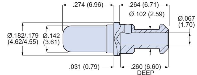
Pin Contact 850-056-0816
