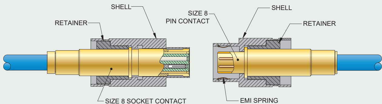
Plug Connector
