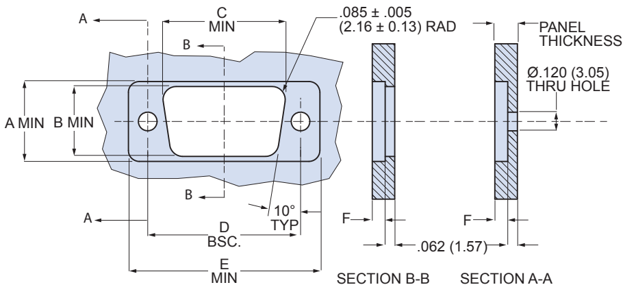
Front Mount Panel Cutout
