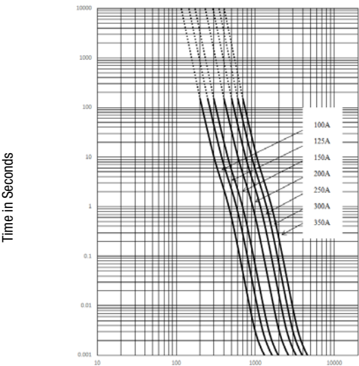
ALO 3148 Bolt-on A and B, 500 VDC
