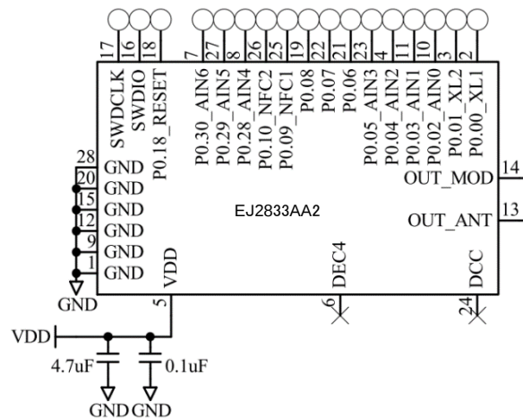
Internal LDO setup
