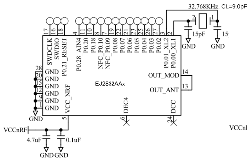
Internal LDO setup with external 32.768kHz X'tal
