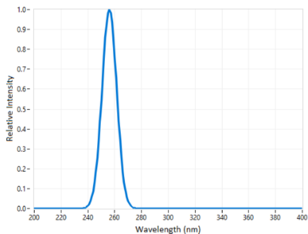
Figure 1. Relative emission intensity vs wavelength T_A = 25^\circ\text{C} , I_f = 20\text{ mA}
