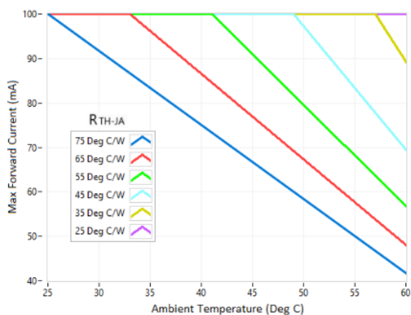
Figure 9. Max Forward current de-rating
