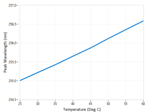
Figure 6. Peak wavelength vs temperature I_F = 20\text{ mA}
