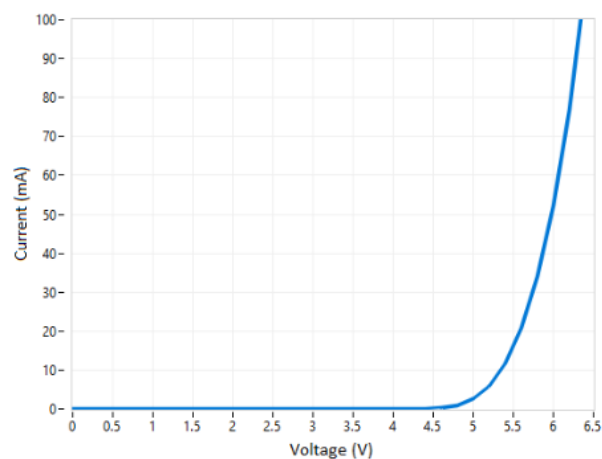
Figure 4. Forward current vs forward voltage T_A = 25^\circ\text{C}
