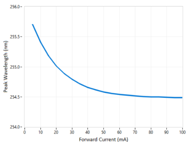
Figure 3. Peak wavelength vs forward current T_A = 25^\circ\text{C}
