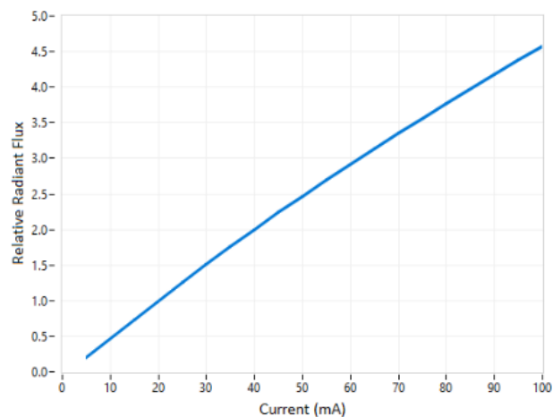
Figure 2. Relative radiant flux vs forward current T_A = 25^\circ\text{C}
