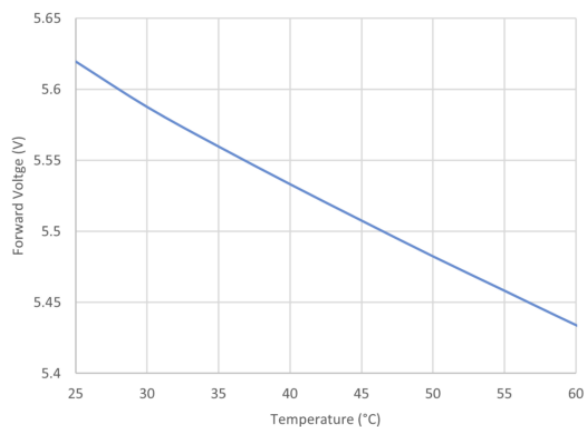
Figure 8. Forward voltage vs temperature ( T_{\text{solder}} ) I_F = 20\text{ mA}
