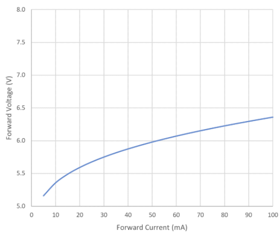
Figure 4. Forward voltage vs forward current T_A=25^\circ\text{C}
