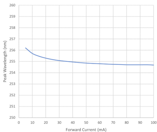
Figure 3. Peak wavelength vs forward current T_A=25^\circ\text{C}
