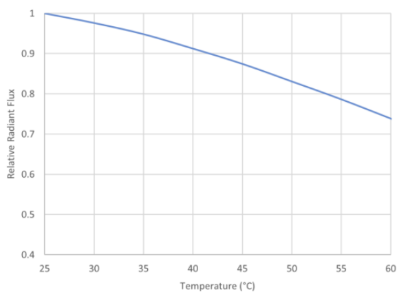
Figure 5. Relative radiant flux vs temperature ( T_{\text{solder}} ) I_F = 20\text{ mA}
