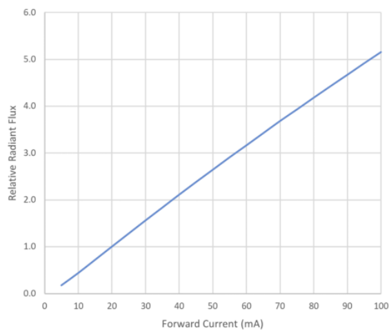
Figure 2. Relative radiant flux vs forward current T_A=25^\circ\text{C}
