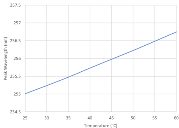
Figure 6. Peak wavelength vs temperature ( T_{\text{solder}} ) I_F = 20\text{ mA}
