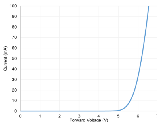
Figure 4. Forward current vs forward voltage T_A = 25^\circ\text{C}
