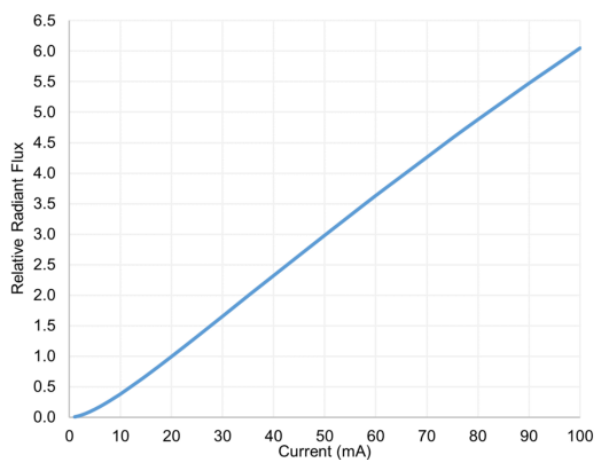
Figure 2. Relative radiant flux vs forward current T_A=25^\circ\text{C}
