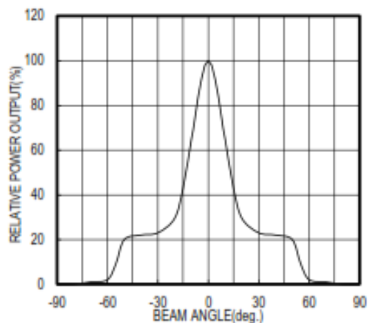
RADIATION PATTERN
