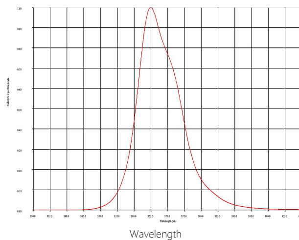
SPECTRAL RESPONSE
