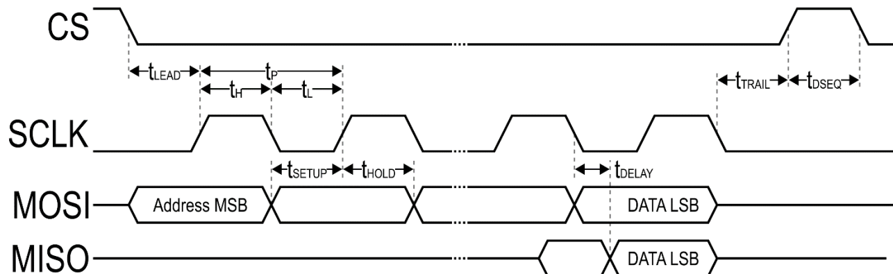
Figure 20 - SPI Slave Interface Timing
