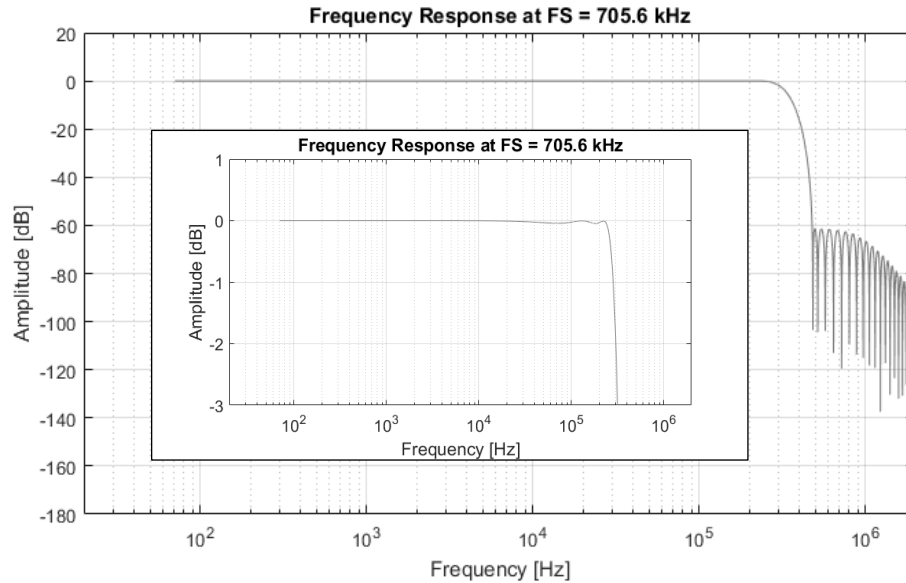
Figure 14 - Minimum Phase 64FS Frequency Response
