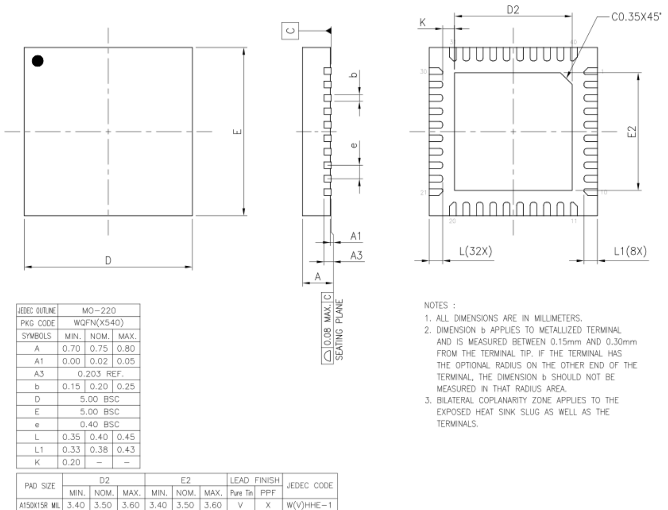
Figure 26 - ES9081 40 QFN Package Dimensions
