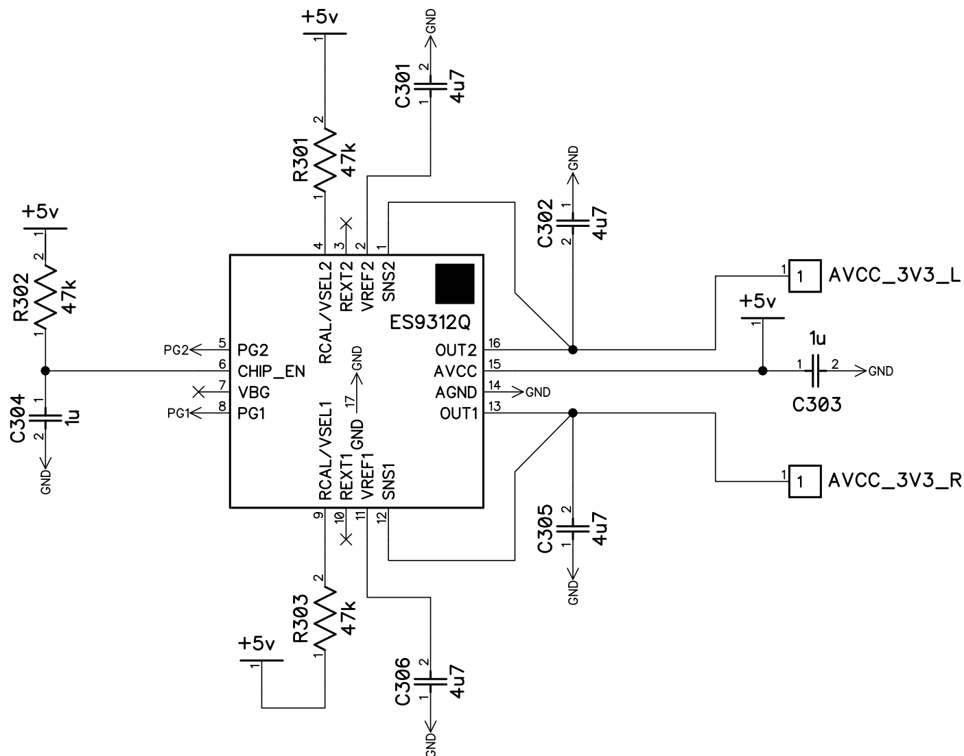
Figure 24 - ES9081 Power Supply Schematic
