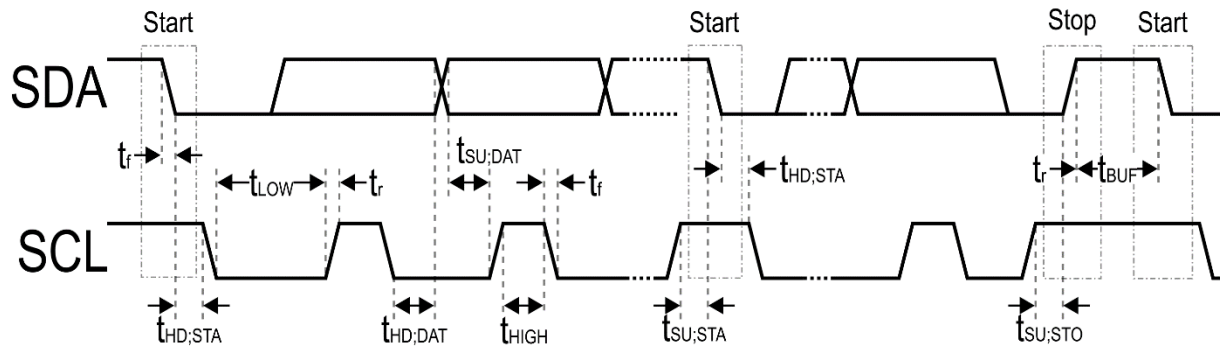
Figure 19 - I 2 C Slave Control Interface Timing
