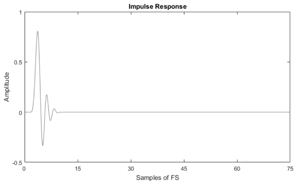
Figure 15 - Minimum Phase 64FS Impulse Response
