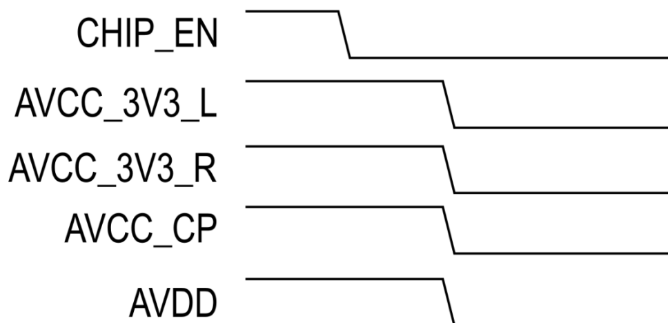
Figure 22 – Recommended Power Down Sequence
