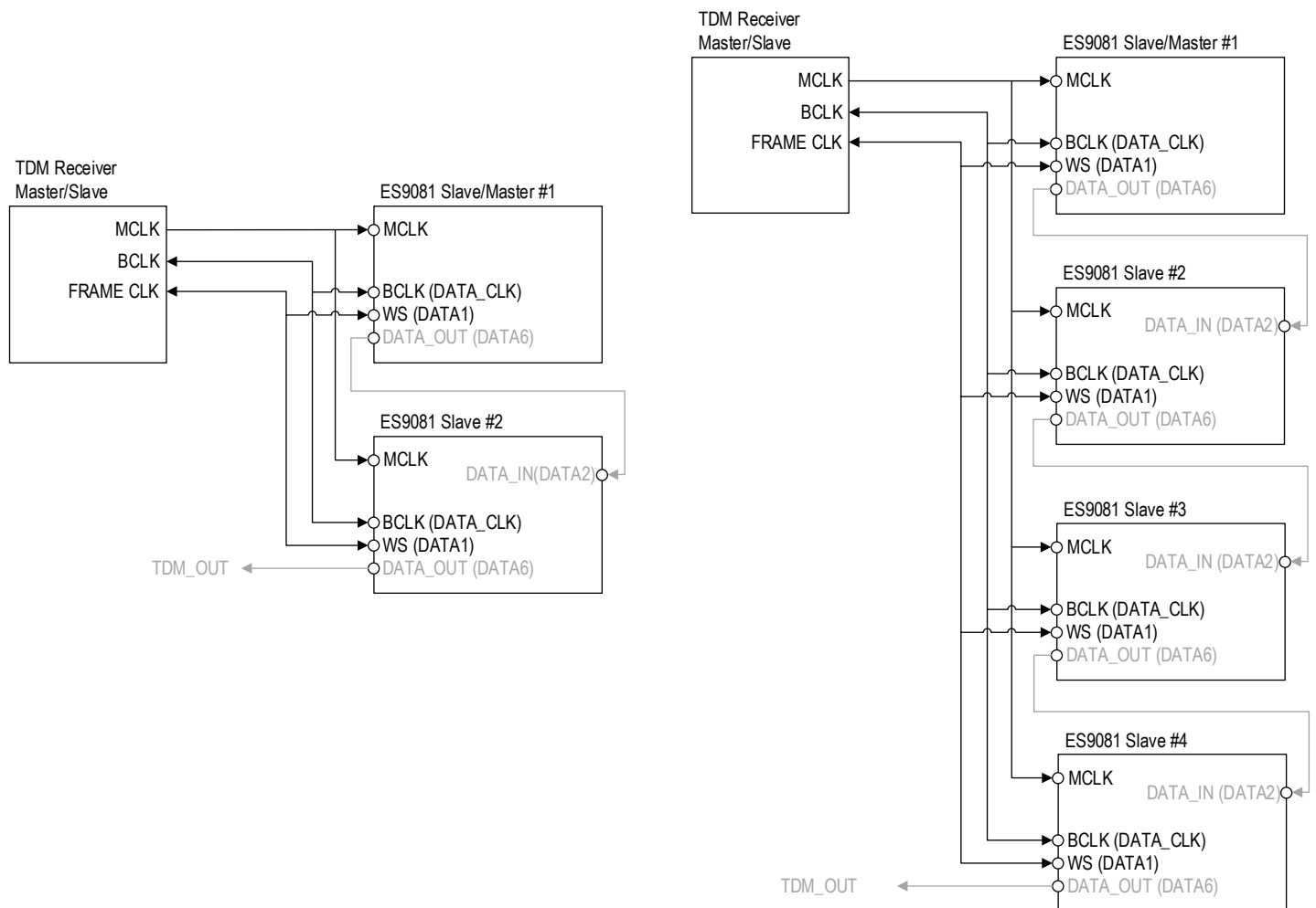
Figure 16 - Example Connection for TDM Decoder Daisy Chain Mode
