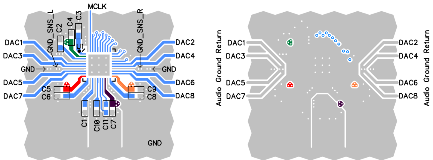
Figure 25 - ES9081 Recommended PCB Layout Guidelines
