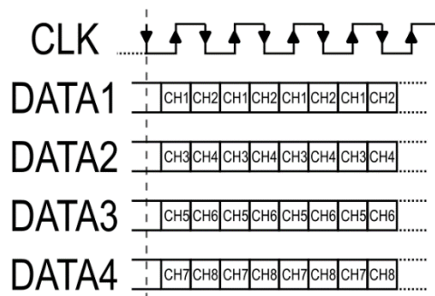
Figure 11 - PDM 8 Channel Format
