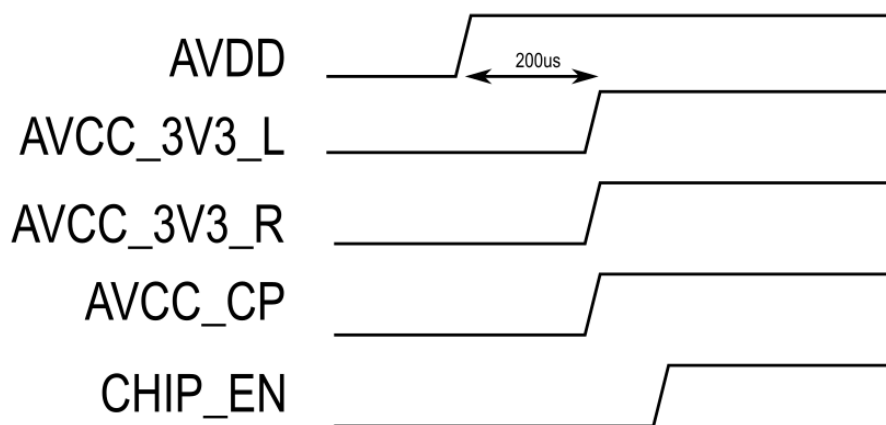
Figure 21 – Recommended Power Up Sequence
