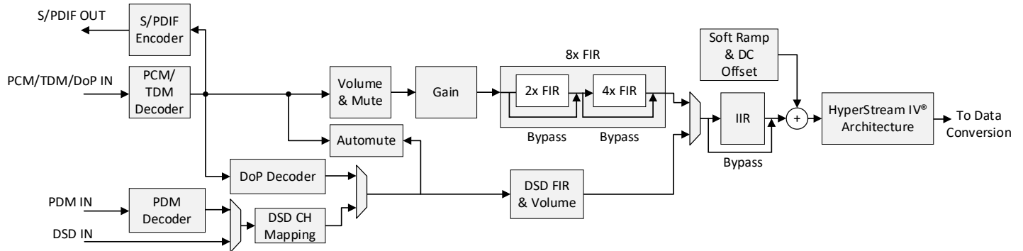
Figure 12 - Digital Signal Path
