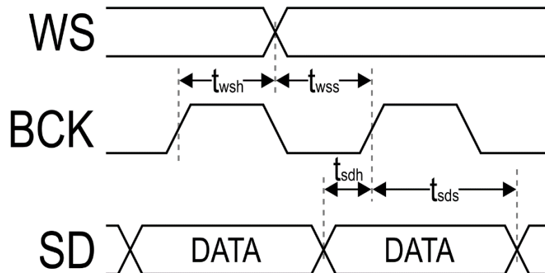
Figure 18 - Bit-Clock and Word-Select Timing
