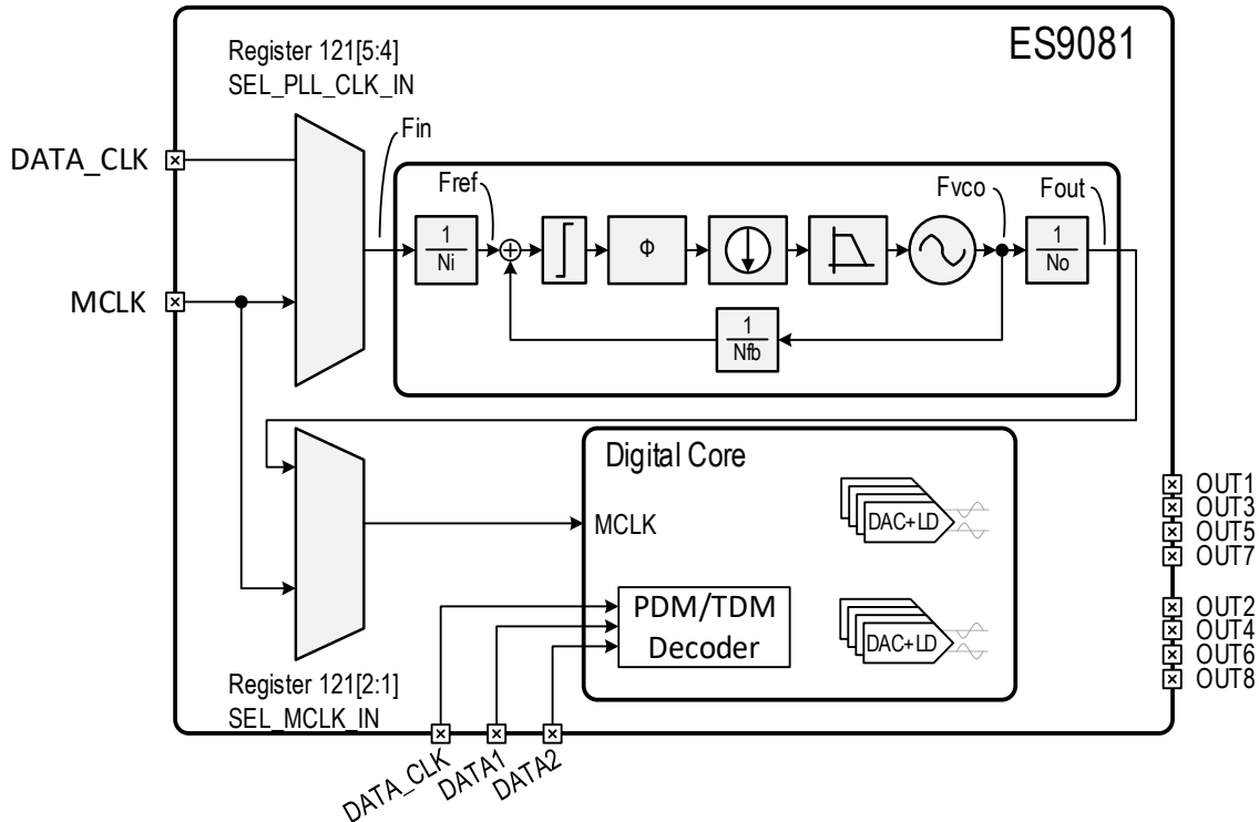
Figure 17 - Functional Block Diagram of ES9081 APLL
