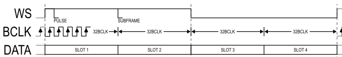
Figure 6 - TDM4 Mode
