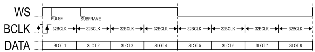
Figure 7 - TDM8 Mode
