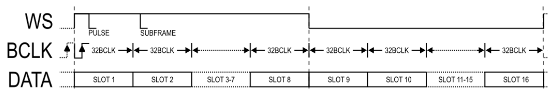
Figure 8 - TDM16 Mode
