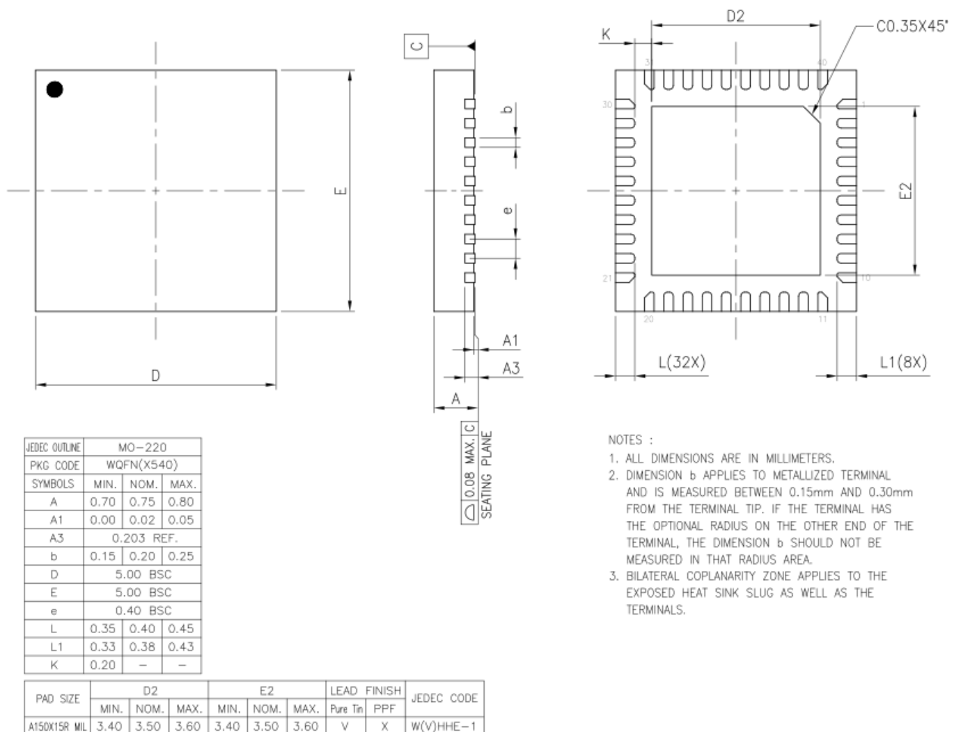
Figure 22 - ES9081 40 QFN Package Dimensions
