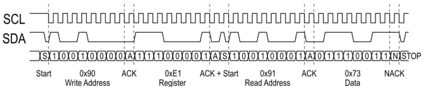
Figure 4 - I 2 C Read Example
