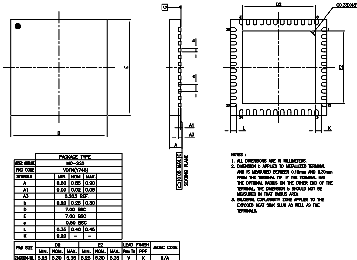
Figure 31 - ES9017Q 48 QFN Package Dimensions
