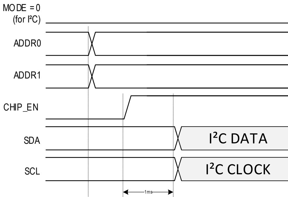
Figure 4 - I 2 C Software Mode Startup Sequence
