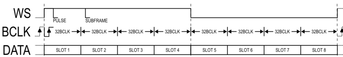
Figure 14 - TDM8 Mode
