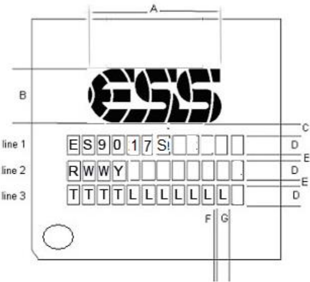
Figure 32 - ES9017S Marking
