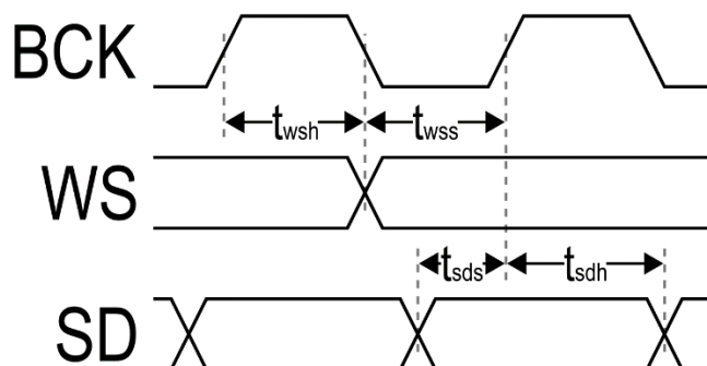
Figure 21 - Bit-Clock and Word-Select Timing
