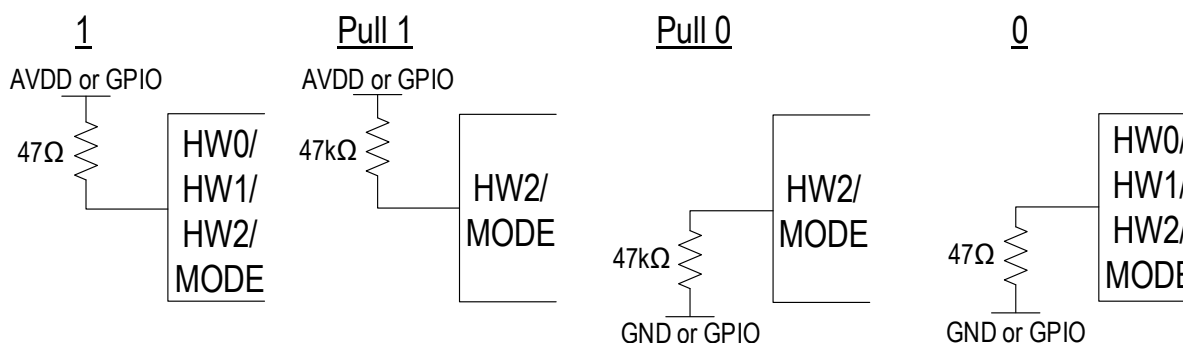
Figure 3 - Hardware Mode Pin Configurations
