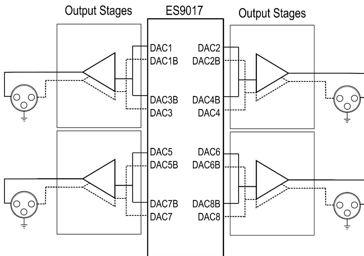
Figure 19 - Example of Channel Combination for 4 Outputs.
