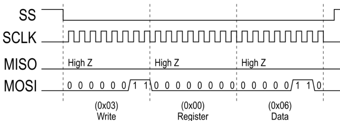
Figure 8 - SPI Single Byte Write
