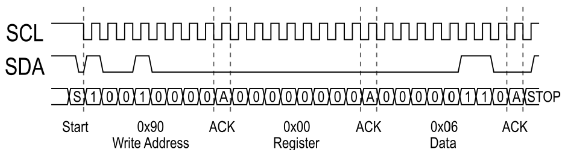
Figure 5 - I 2 C Write Example
