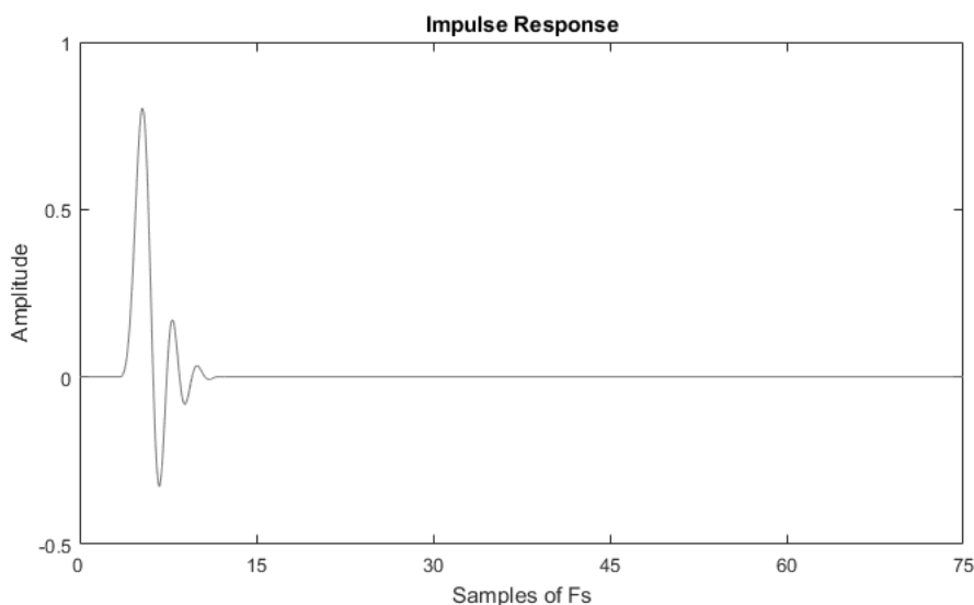
Figure 18 – Minimum Phase 64FS Impulse Response
