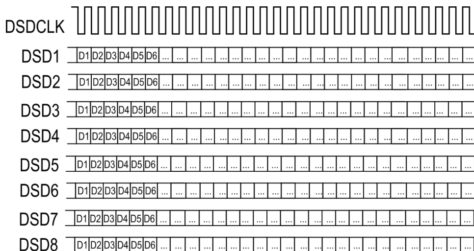
Figure 16 - DSD Format, 1-bit stream
