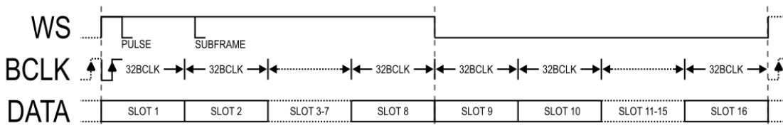
Figure 15 - TDM16 Mode
