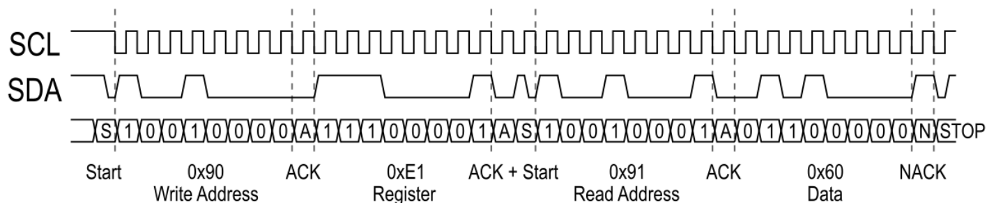
Figure 6 - I 2 C Read Example
