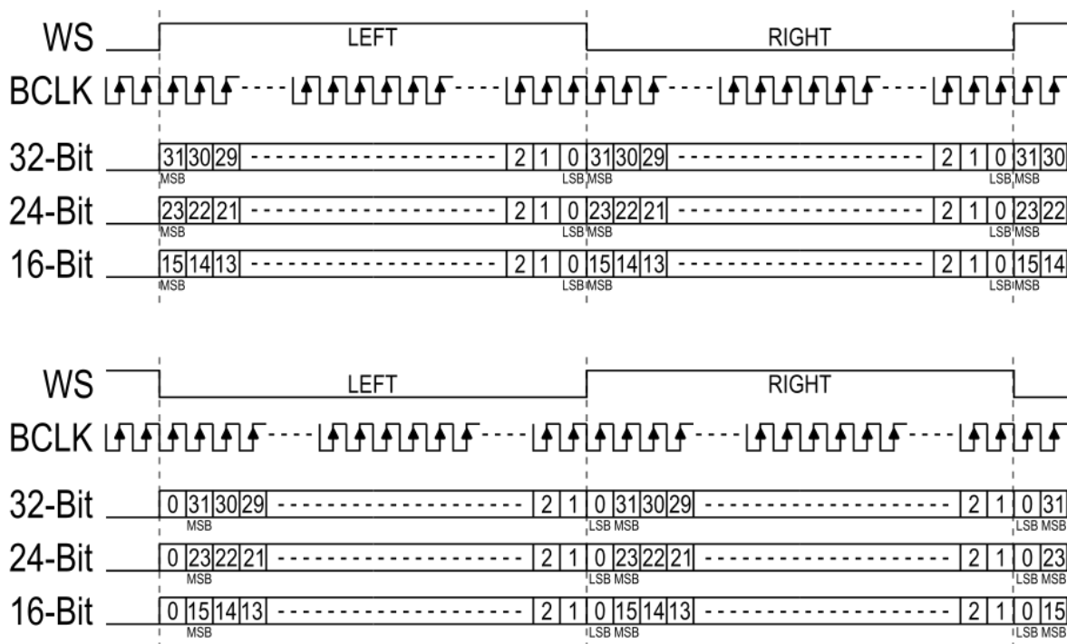
Figure 12 - LJ (top) & I 2 S (bottom) for 16, 24, and 32-bit Word Widths
