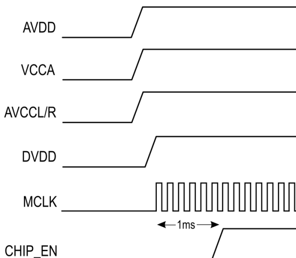
Figure 24 - Power up sequence
