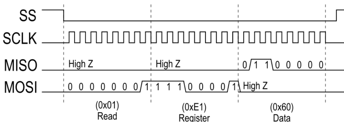
Figure 7 - SPI Single Byte Read
