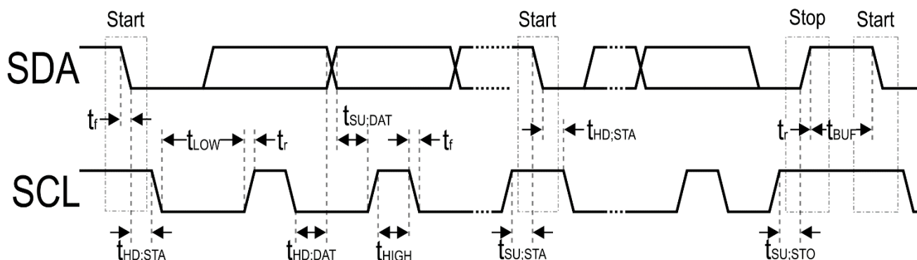
Figure 22 - I 2 C Slave Control Interface Timing
