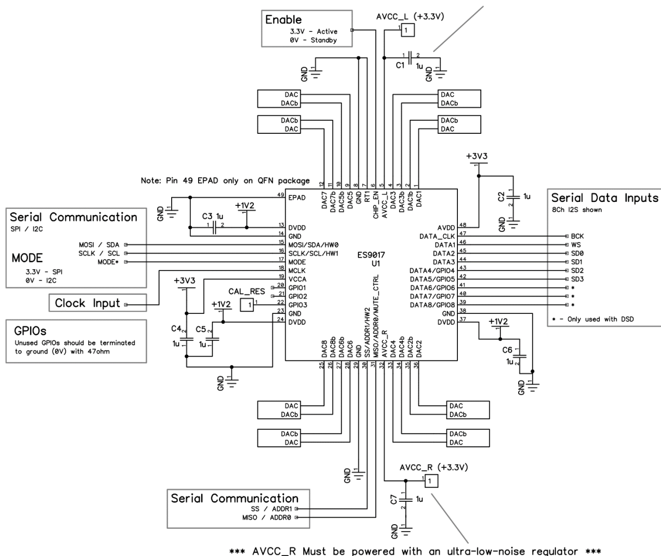
Figure 27 - ES9017Q Software Mode Reference Schematic
