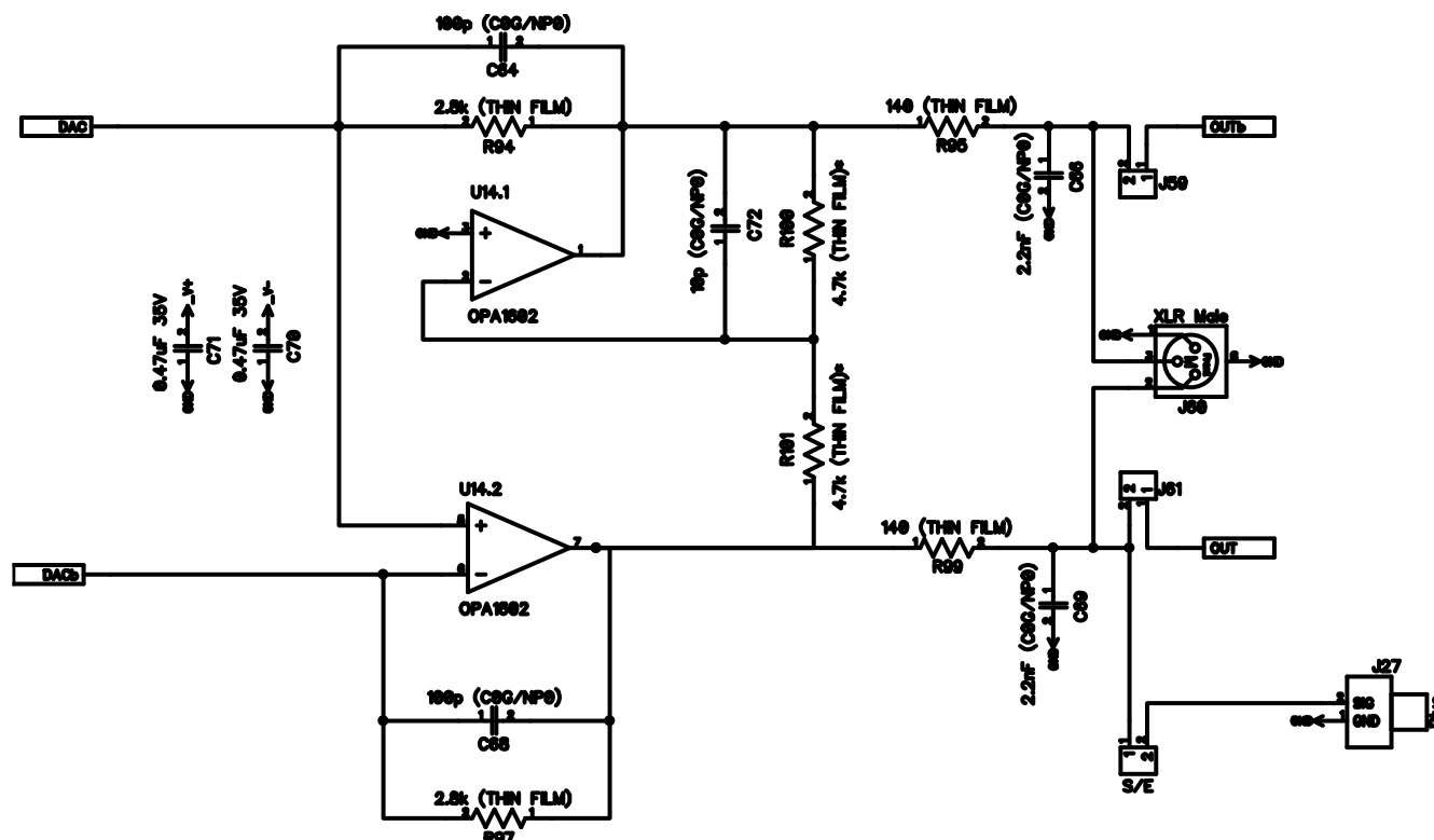
Figure 28 - ES9017 Output Stage Schematic
