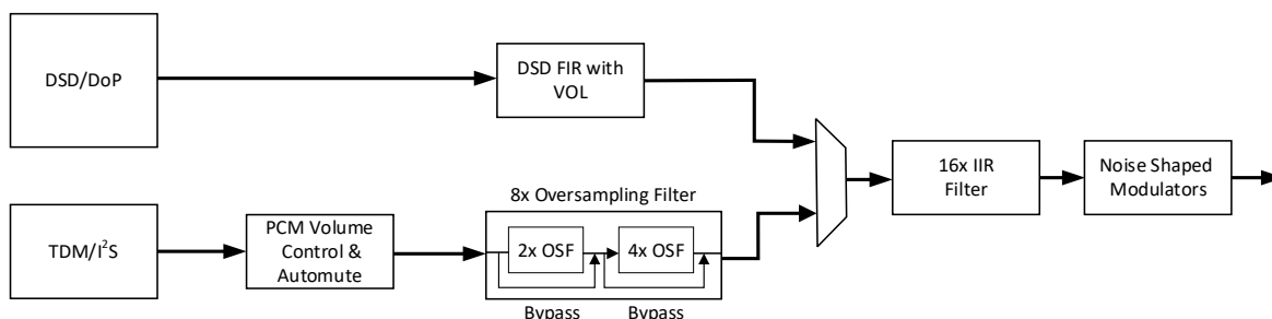
Figure 10 - Digital Signal Path
