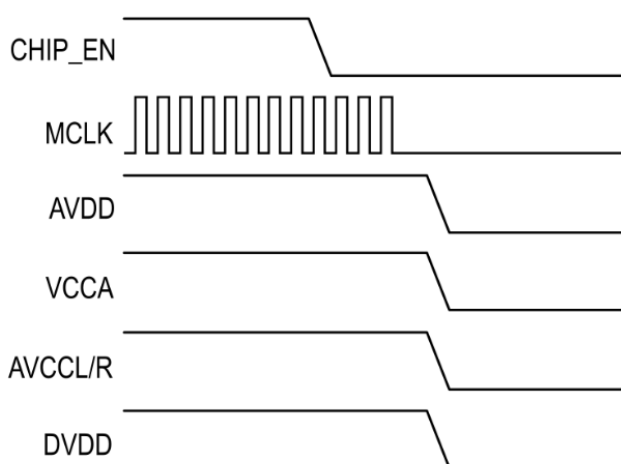
Figure 25 - Power down sequence
