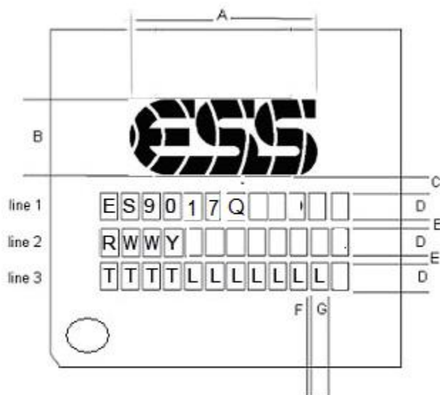
Figure 33 - ES9017Q Marking
