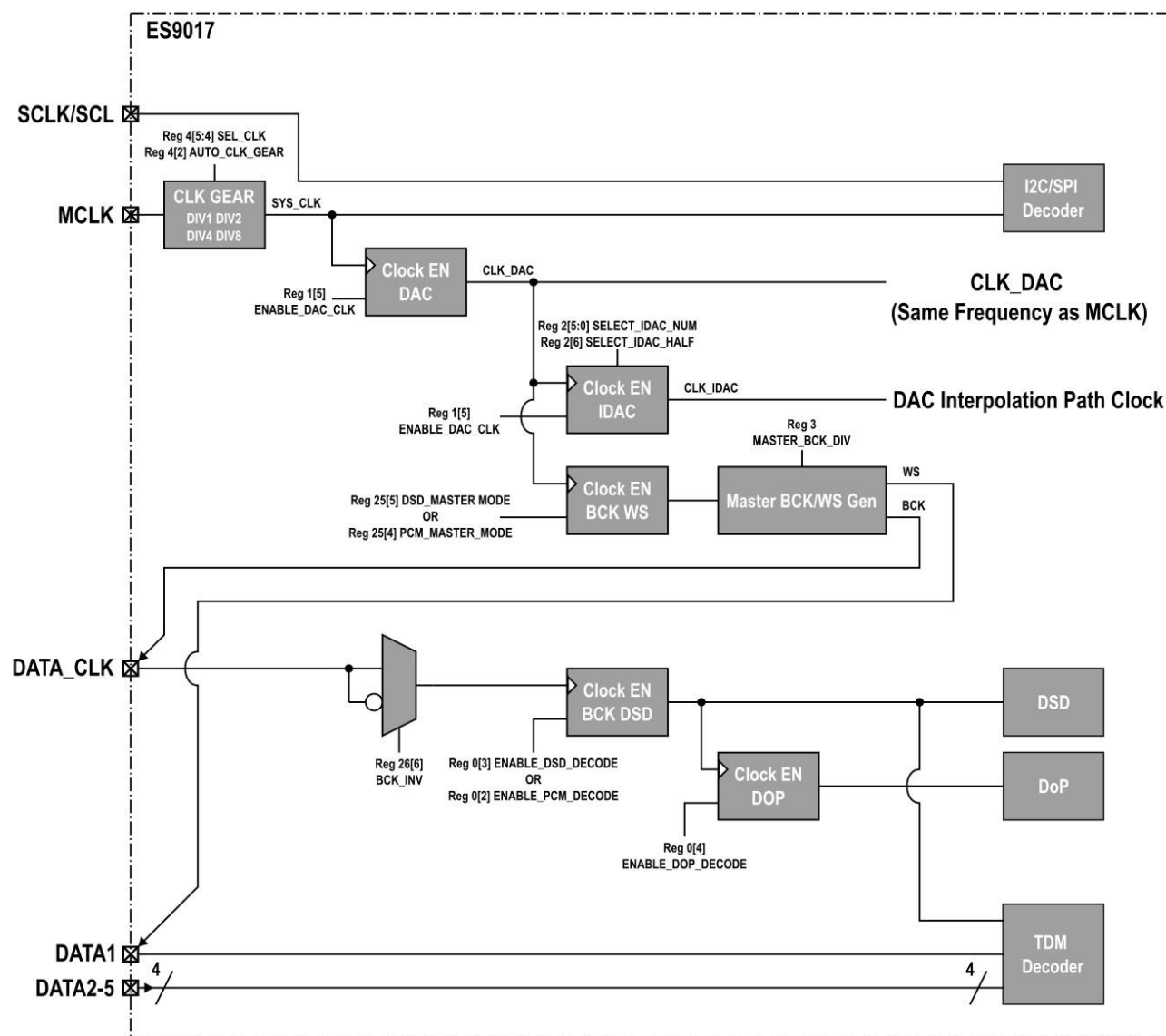
Figure 11 - Internal clock distribution diagram for ES9017
