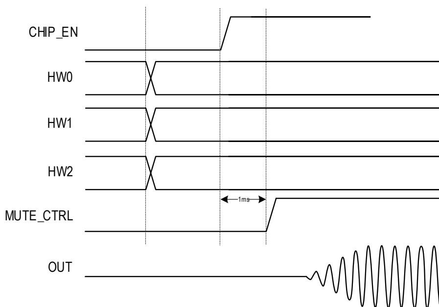
Figure 9 - Hardware Mode Startup Sequence
