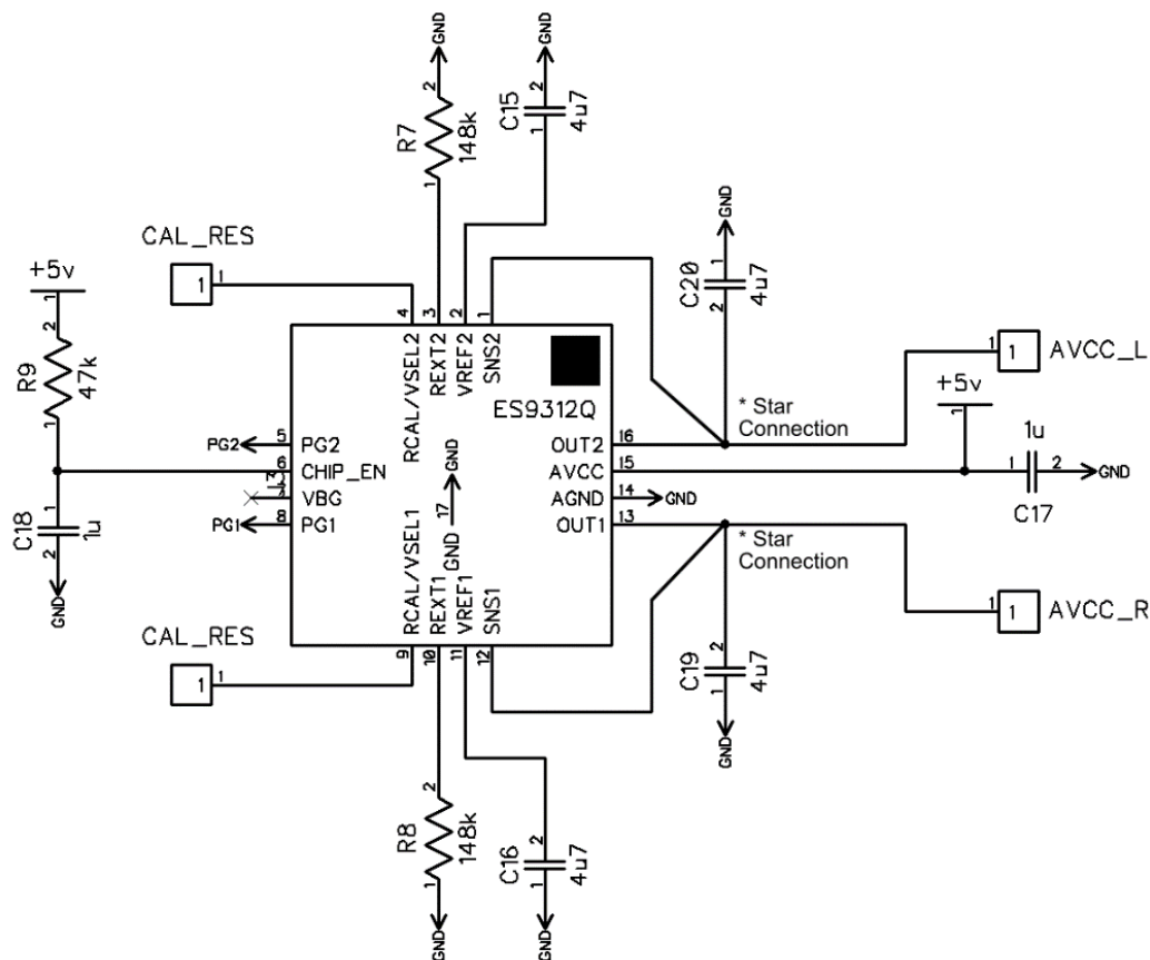
Figure 29 - ES9017 Power Supply Schematic
