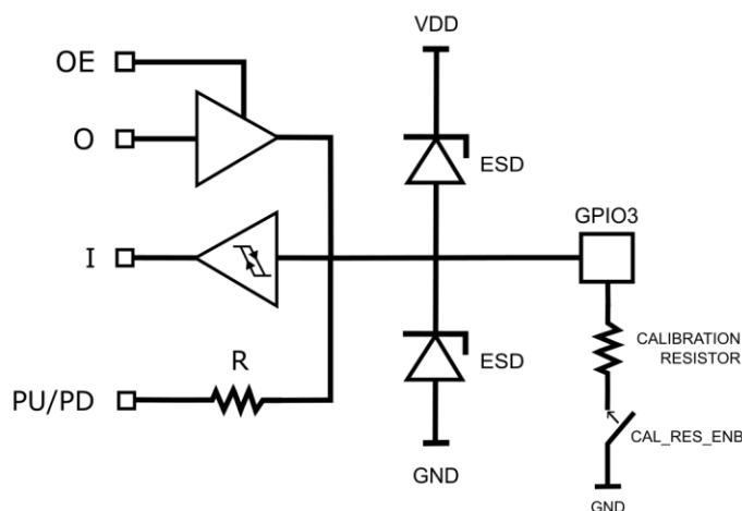
Figure 20 - GPIO3 Digital I/O with Calibration Resistor
