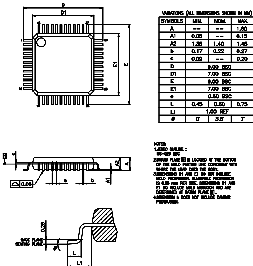
Figure 30 - ES9017S 48 QFP Package Dimensions
