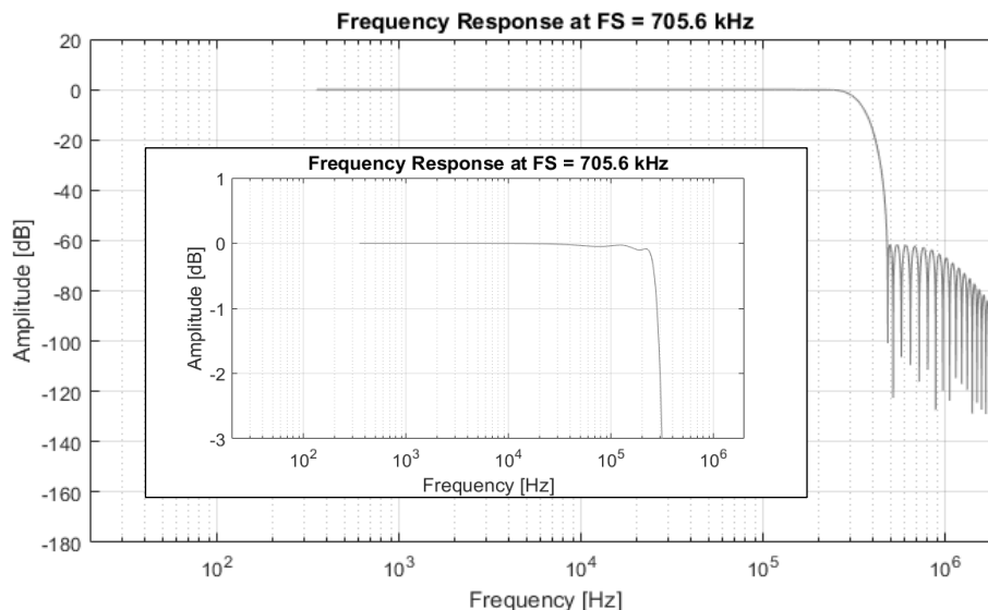
Figure 17 - Minimum Phase 64FS Frequency Response
