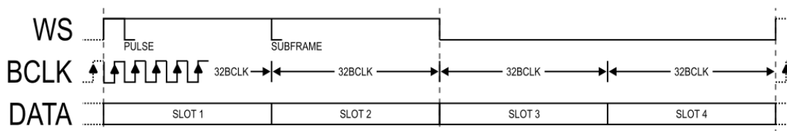
Figure 13 - TDM4 Mode
