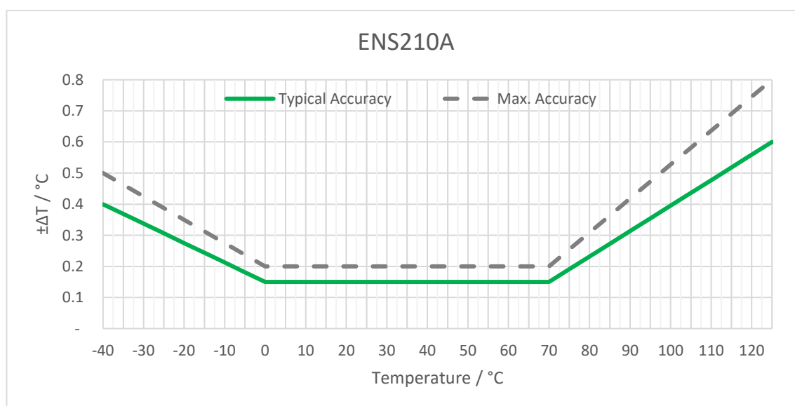
Figure 5: Typical and maximum temperature accuracy
