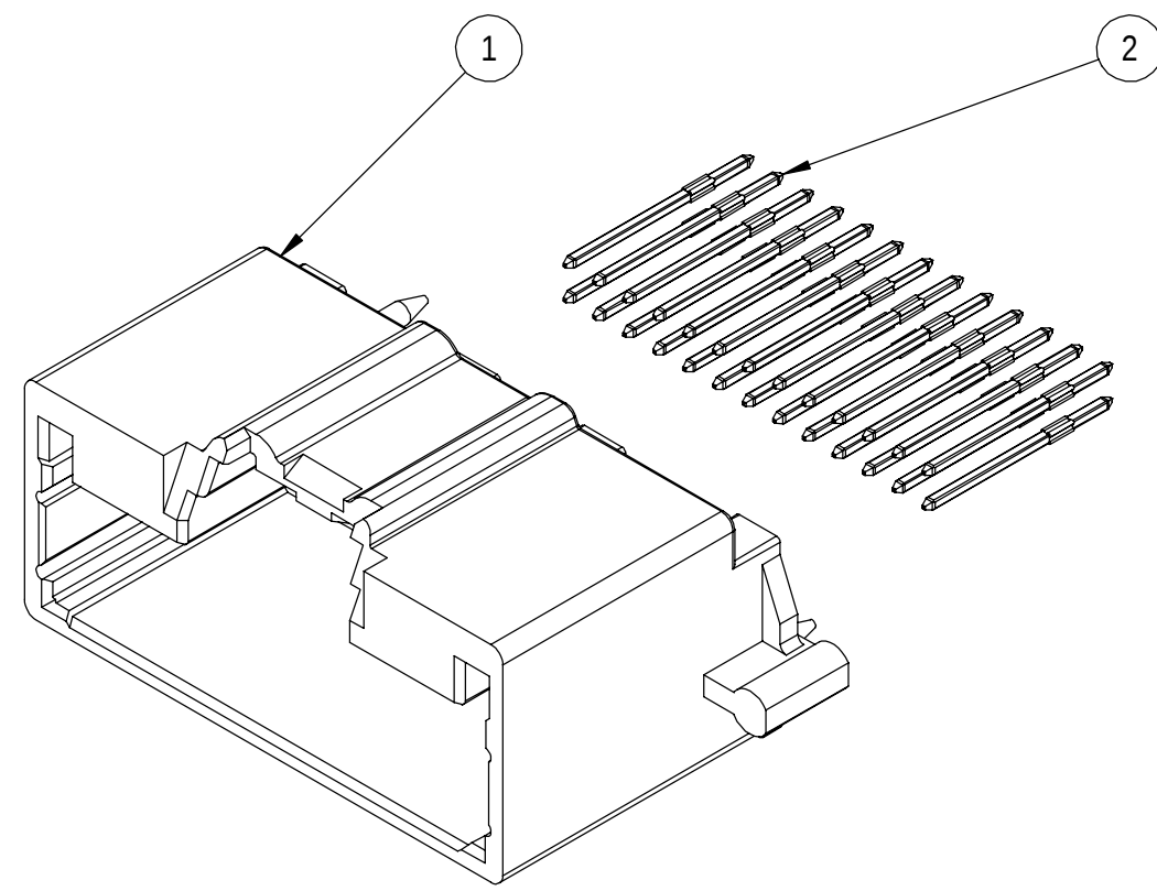
EXPLODED VIEW
