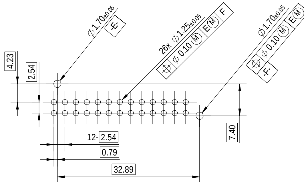
PCB FOOTPRINT
