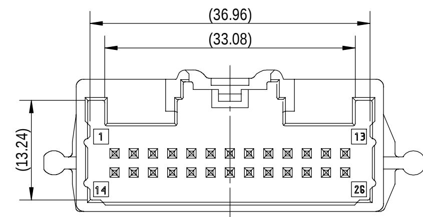
7386-9376-3R KEYWAY A
