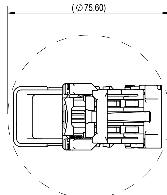
RECOMENDED PASS-THROUGH HOLE DIMENSION WITH 7174-1436 (1mm CLEARANCE ALL AROUND) (1/1)
