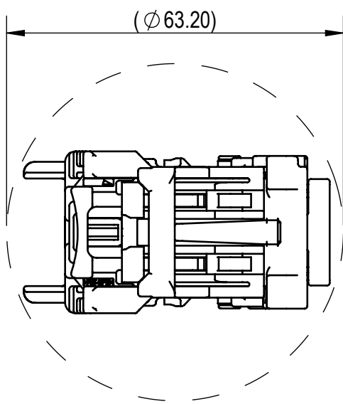
RECOMENDED PASS-THROUGH HOLE DIMENSION (1mm CLEARANCE ALL AROUND) (1/1)
