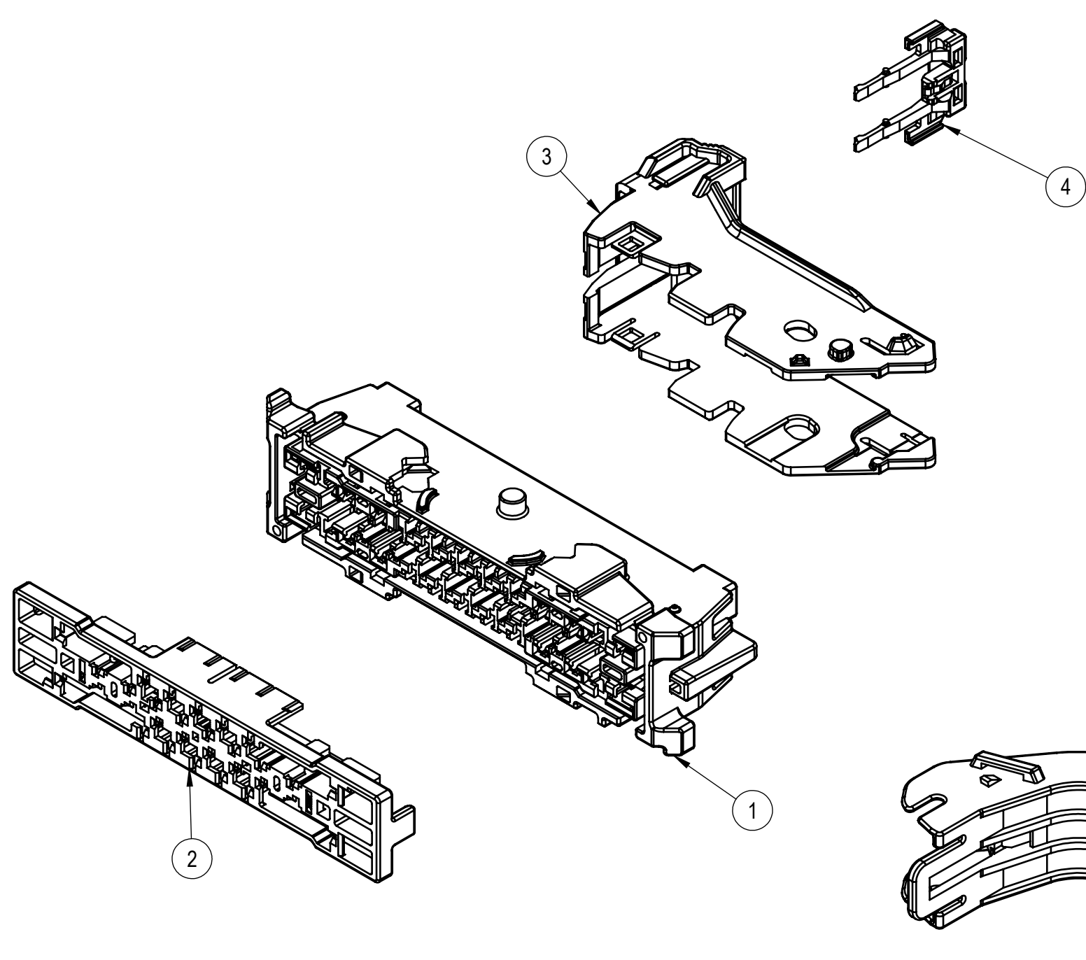
EXPLODED VIEW (1/1)
