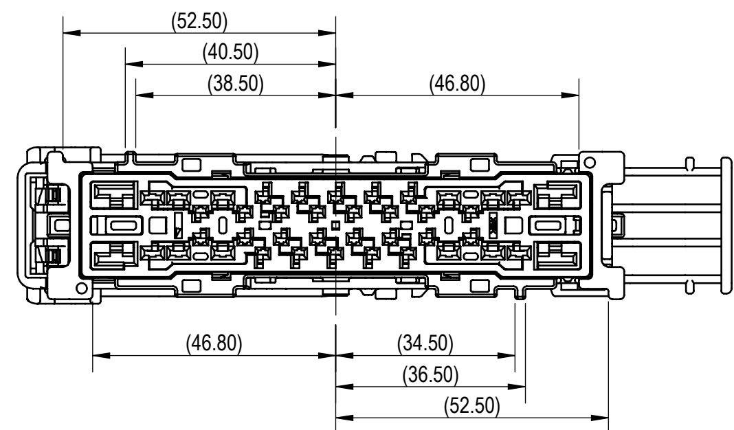
7298-5662-40 KEYWAY B
