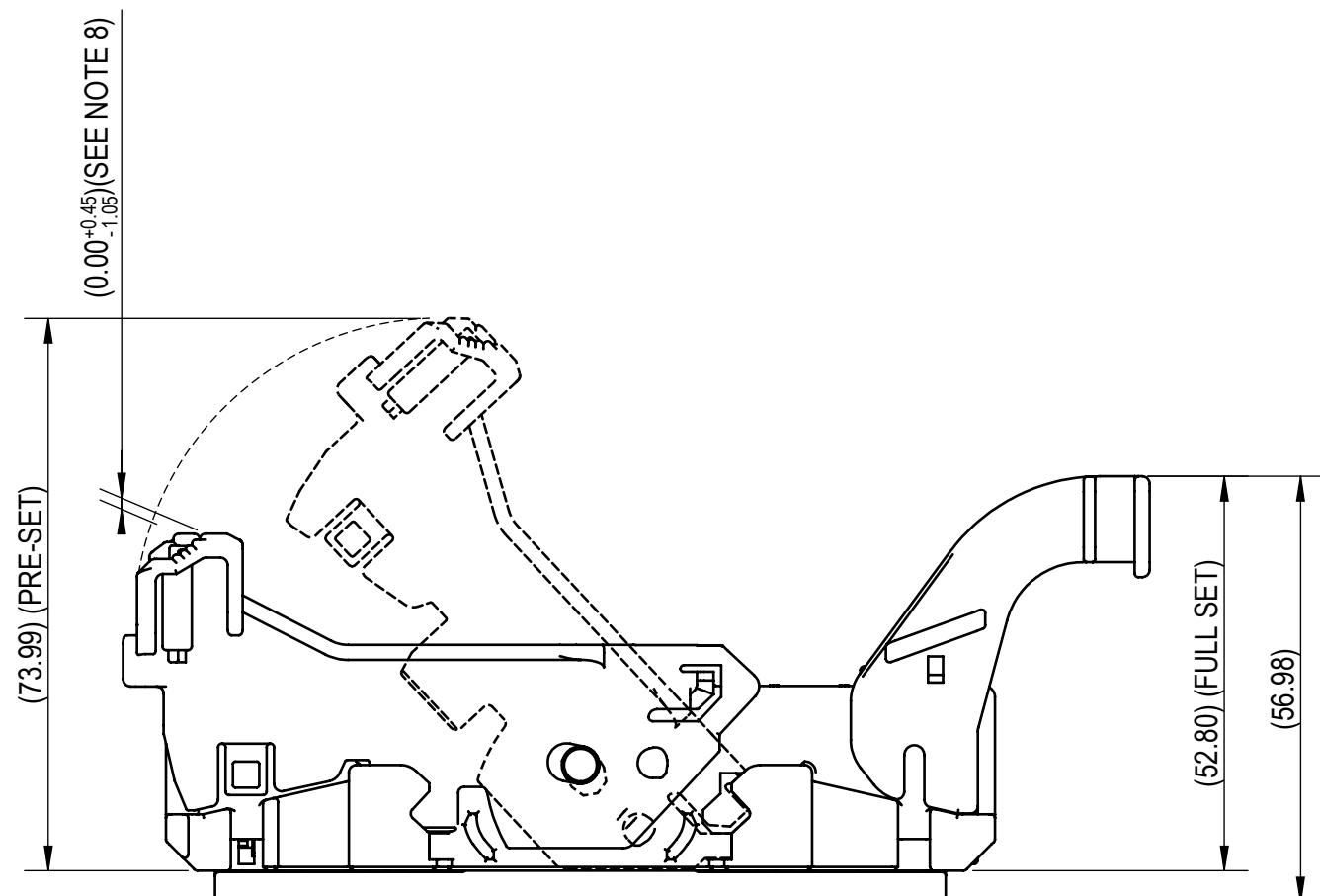
7298-5662-40 KEYWAY B
