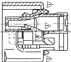
SEC. B-B
