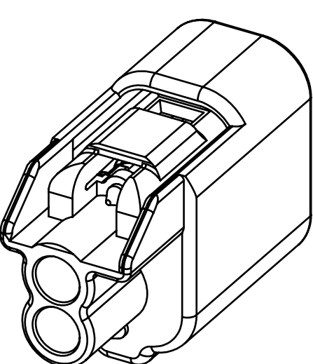
△ REAR ISOMETRIC VIEW (2/1)
