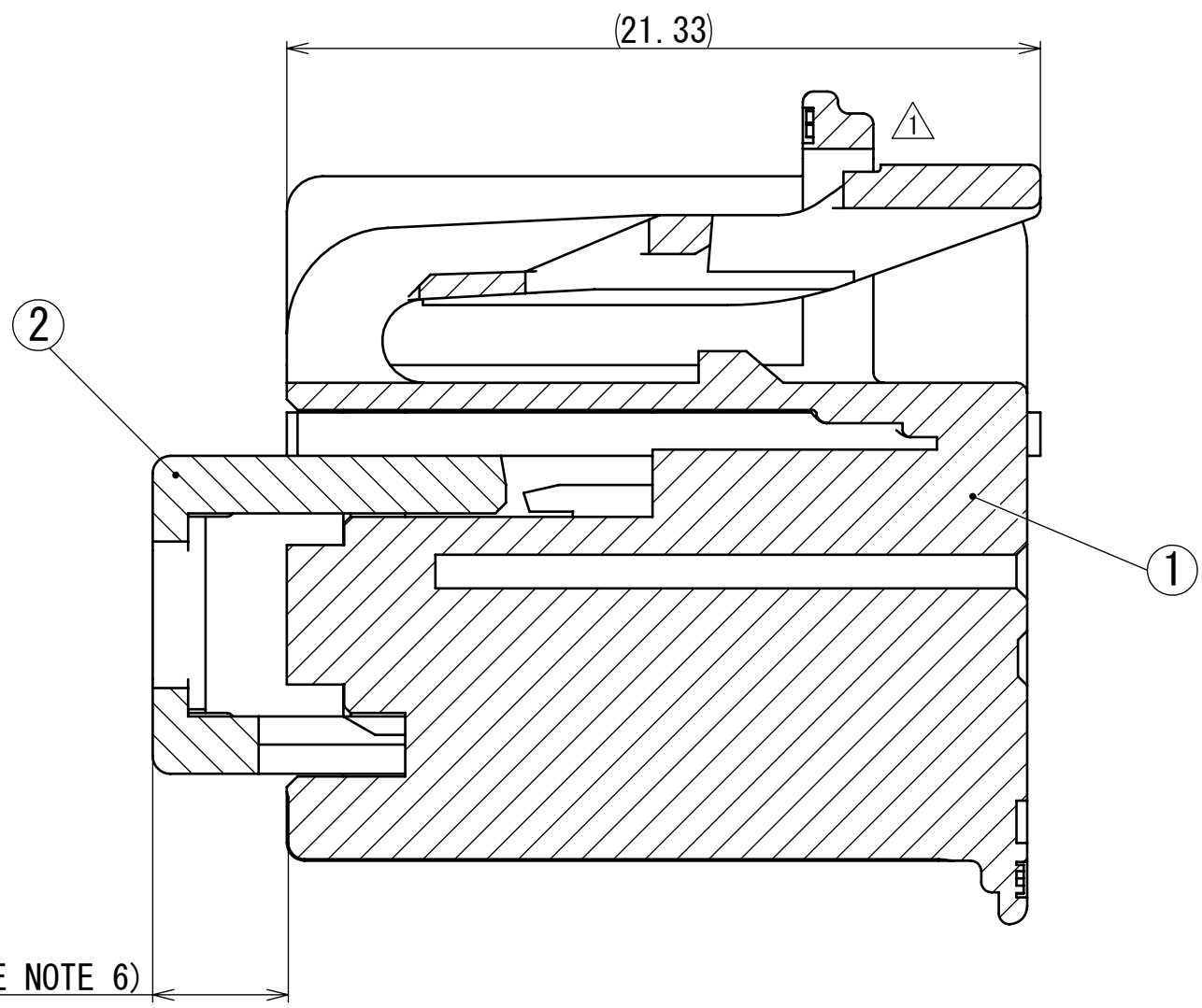
SECTION A-A SUB-ASSEMBLY WITHOUT CPA
