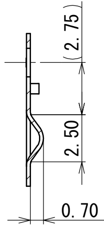
SEC. C-C
