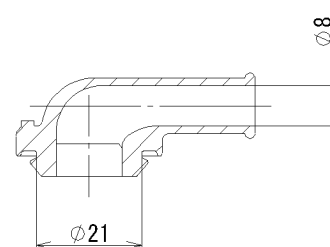
SECT AA
