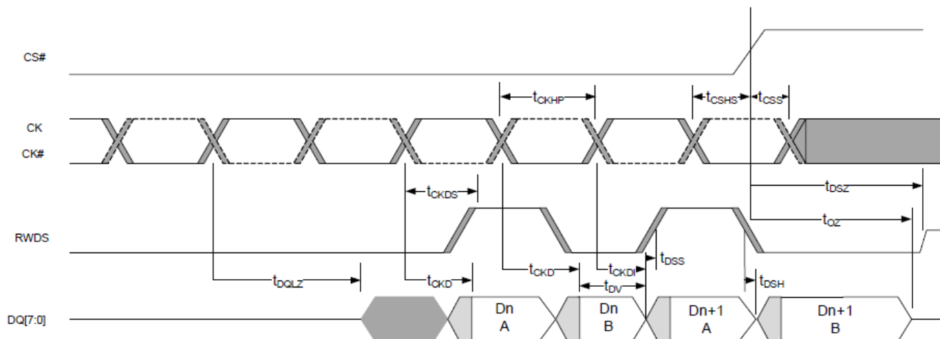
Figure 10.7 Read Timing Diagram — Data valid timing
