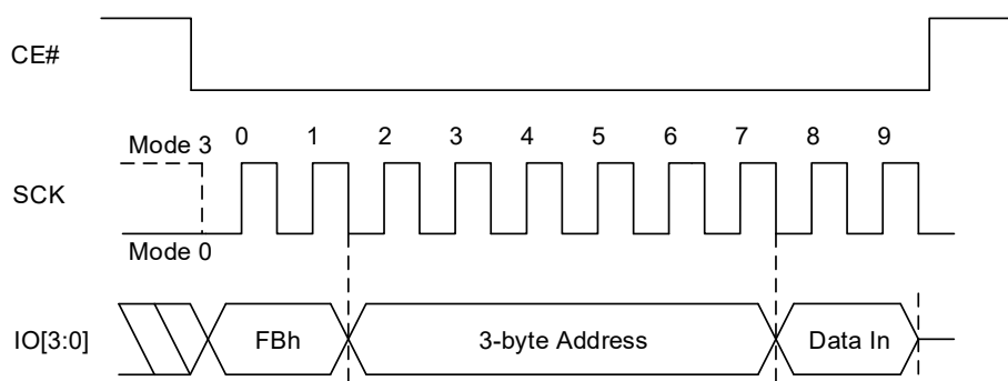
Figure 8.117 Write DYB Sequence In QPI Mode (FBh [EXTADD=0], 3-byte address)
