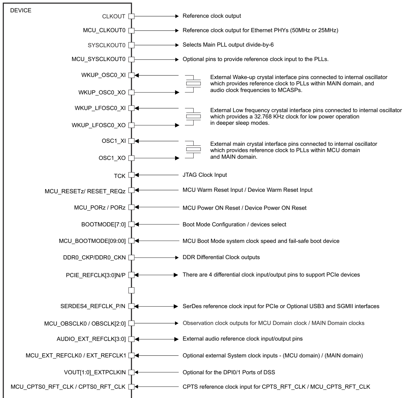
Figure 6-22. Input Clocks Interface
