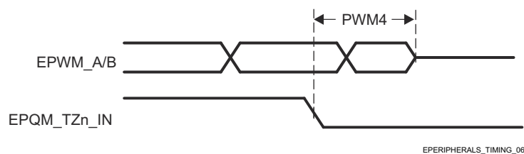
Figure 6-60. EPWM_A/B and ePWM_TZn_IN Hi-Z Input Timings
