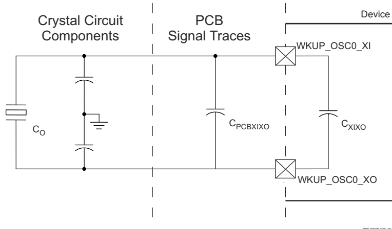
Figure 6-26. Shunt Capacitance
