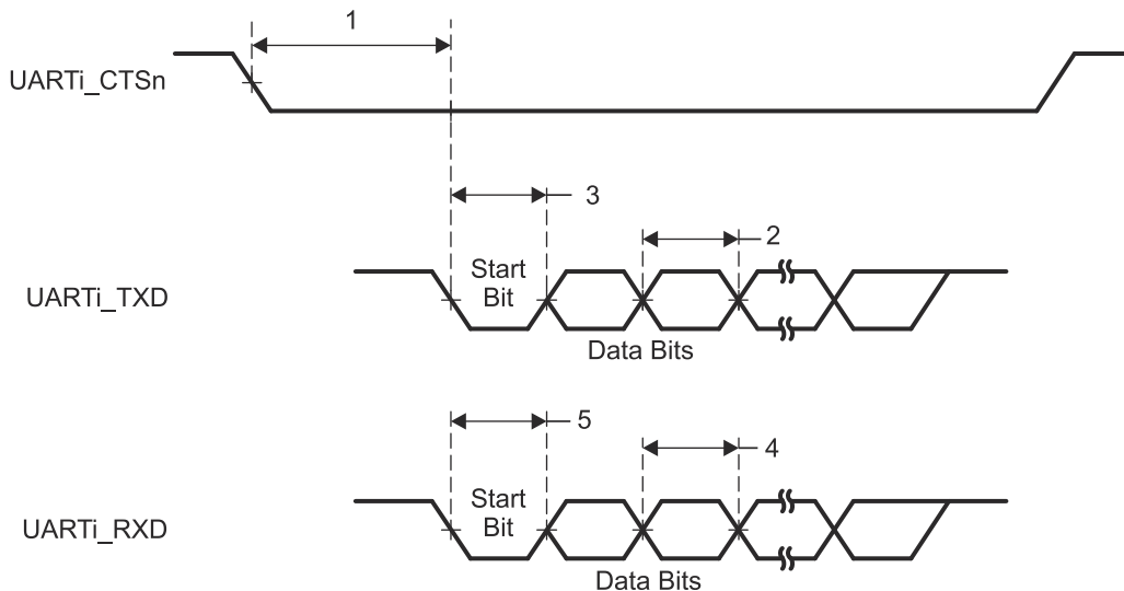
Figure 6-120. UART Timing
