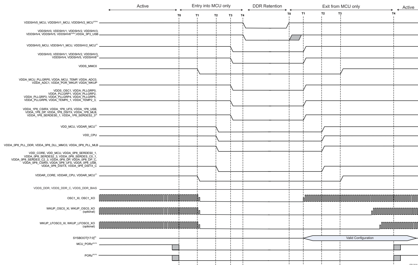
Figure 6-8. Entry and Exit of DDR Retention Sequencing
