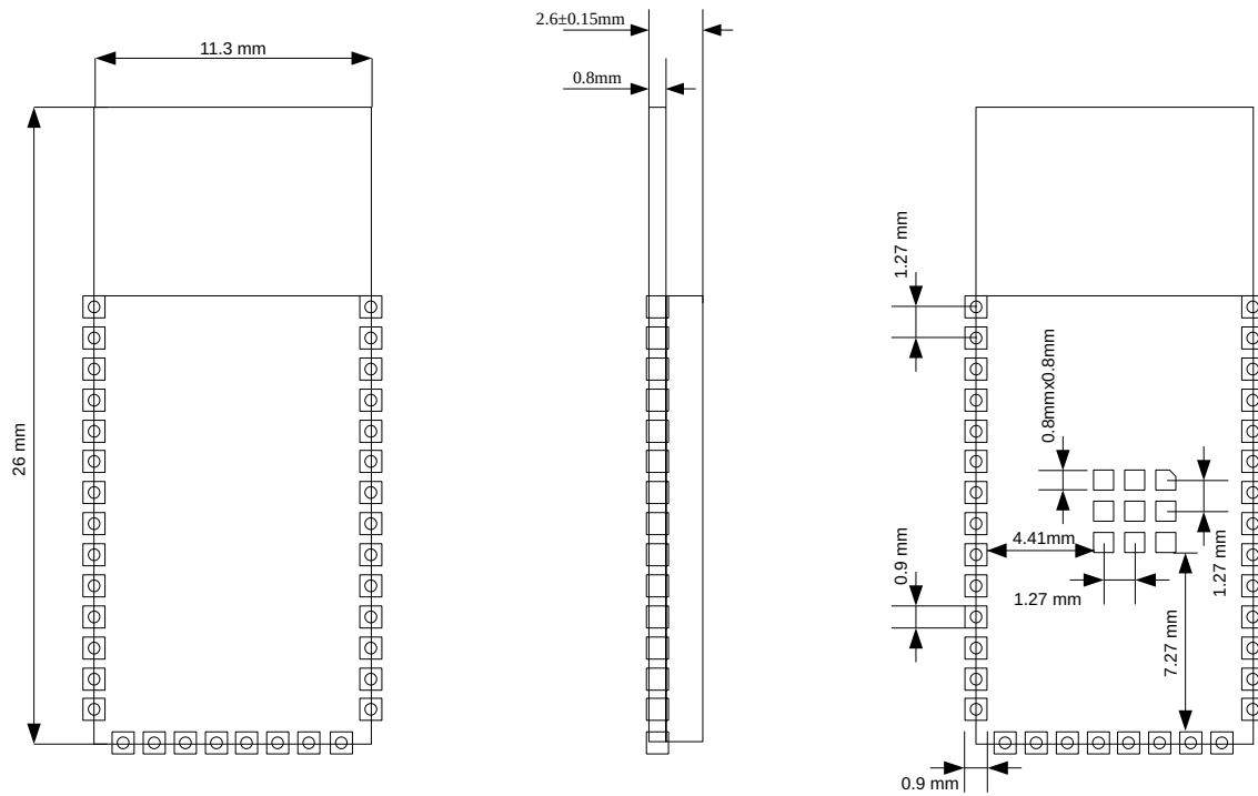
Figure 1-3 Package of ML7218D1-MERCURY-MO-PE11
