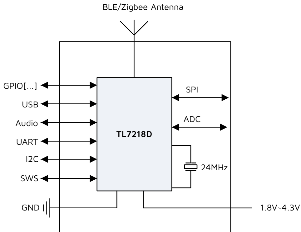
Figure 1-1 Function Block Diagram of the Module
