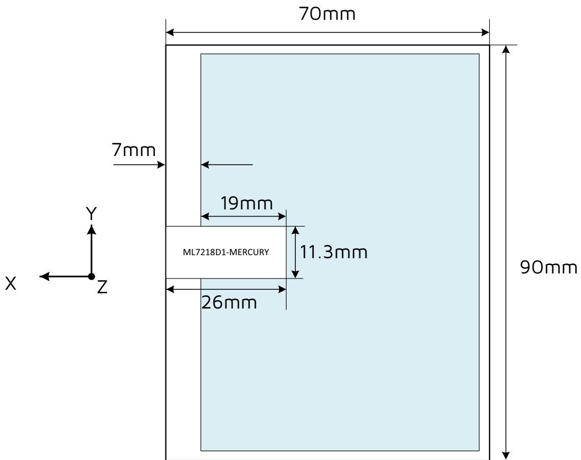
Figure 4-1 RF Layout and Ground Plane
