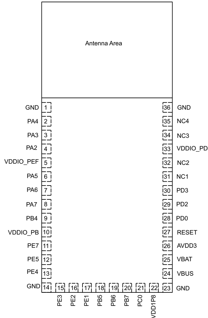
Figure 1-5 Pin Assignment
