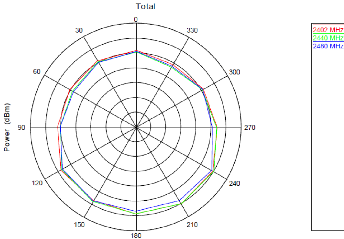
Figure 4-2 Antenna Pattern of X-Y Plane
