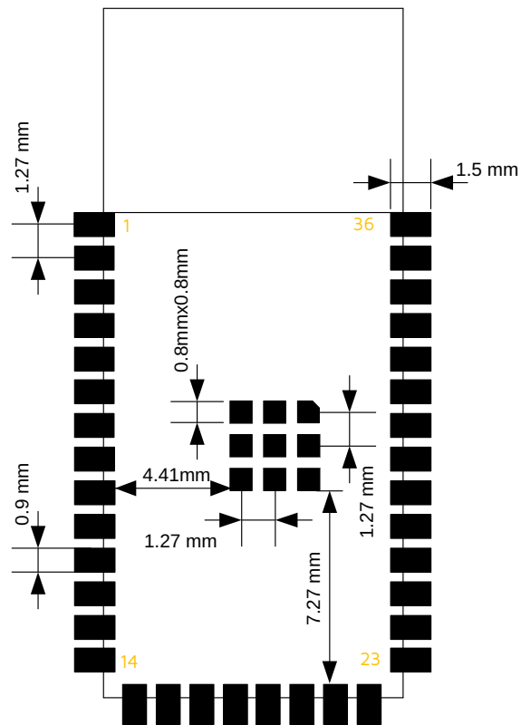
Figure 1-4 PCB land pattern of ML7218D1-MERCURY-MO-PE11
