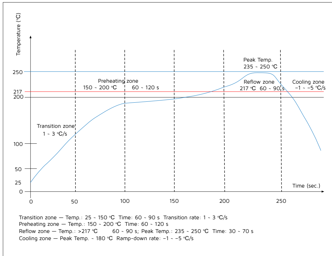
Figure 2-1 Reflow Profile
