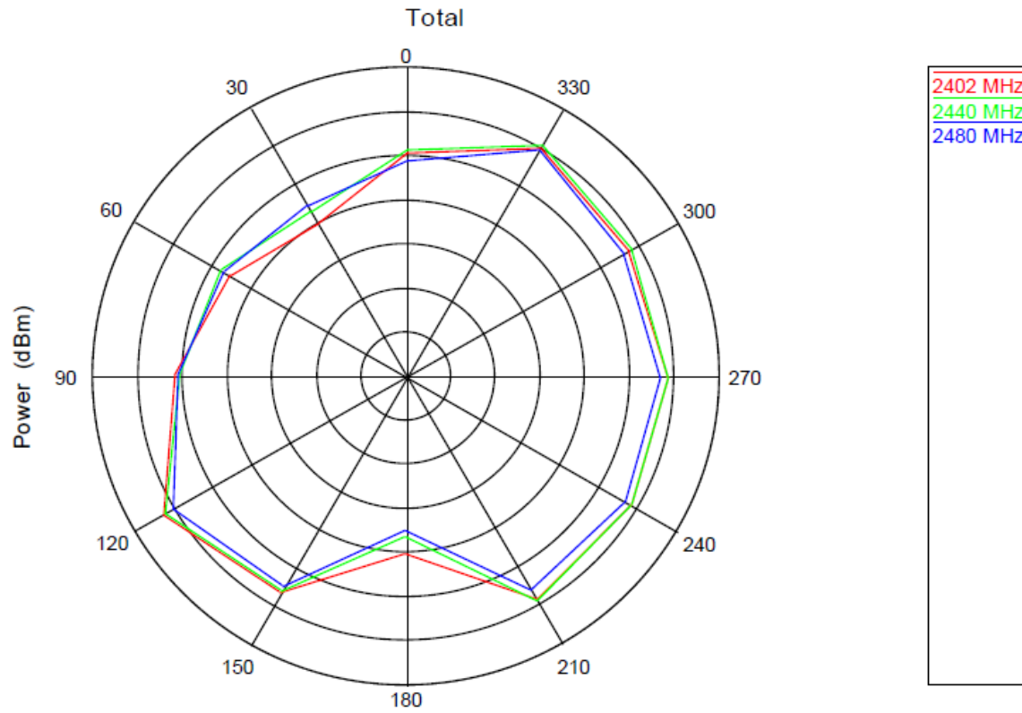
Figure 4-4 Antenna Pattern of Y-Z Plane
