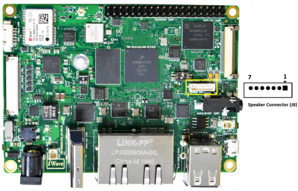
Figure 18: Speaker Header
