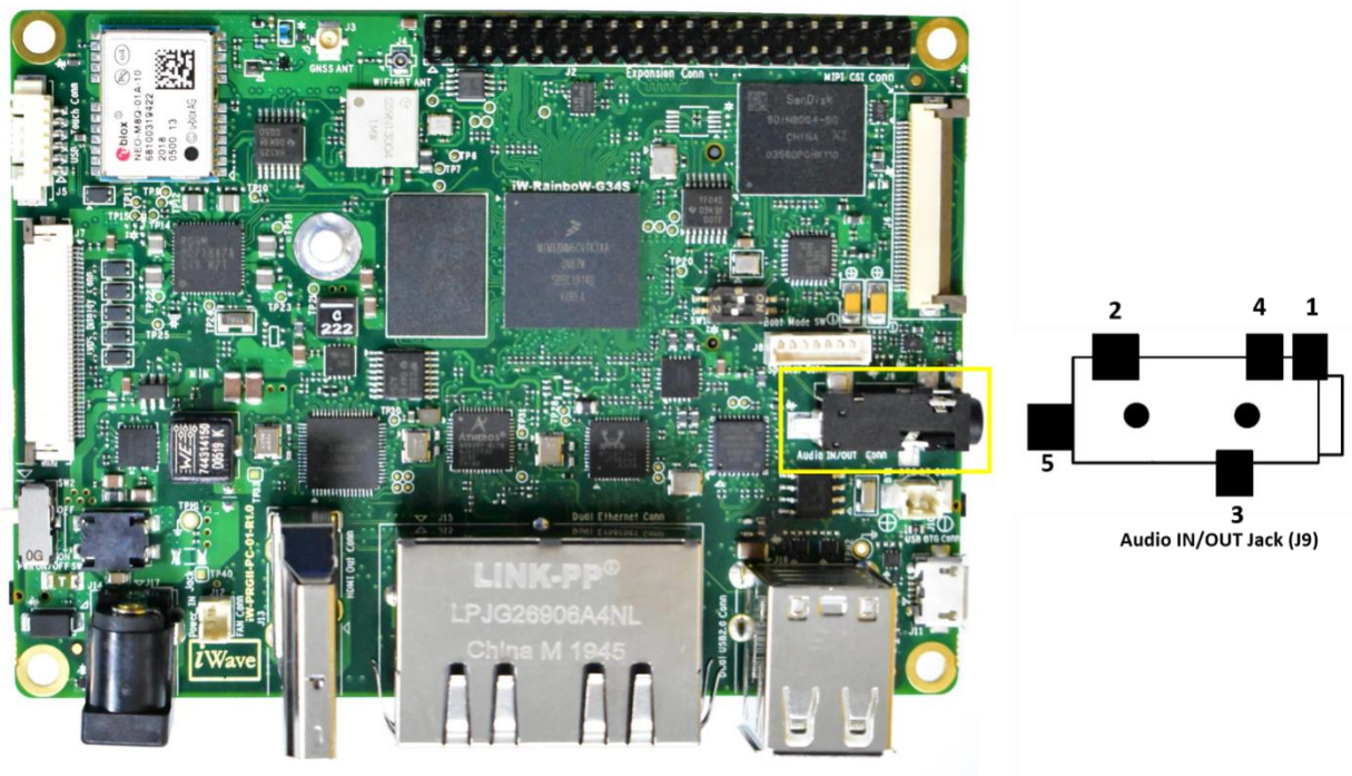
Figure 17: Audio IN/OUT Jack
