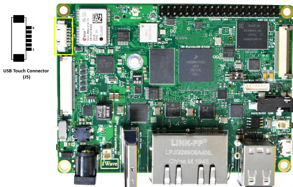
Figure 21: USB Touch Connector
